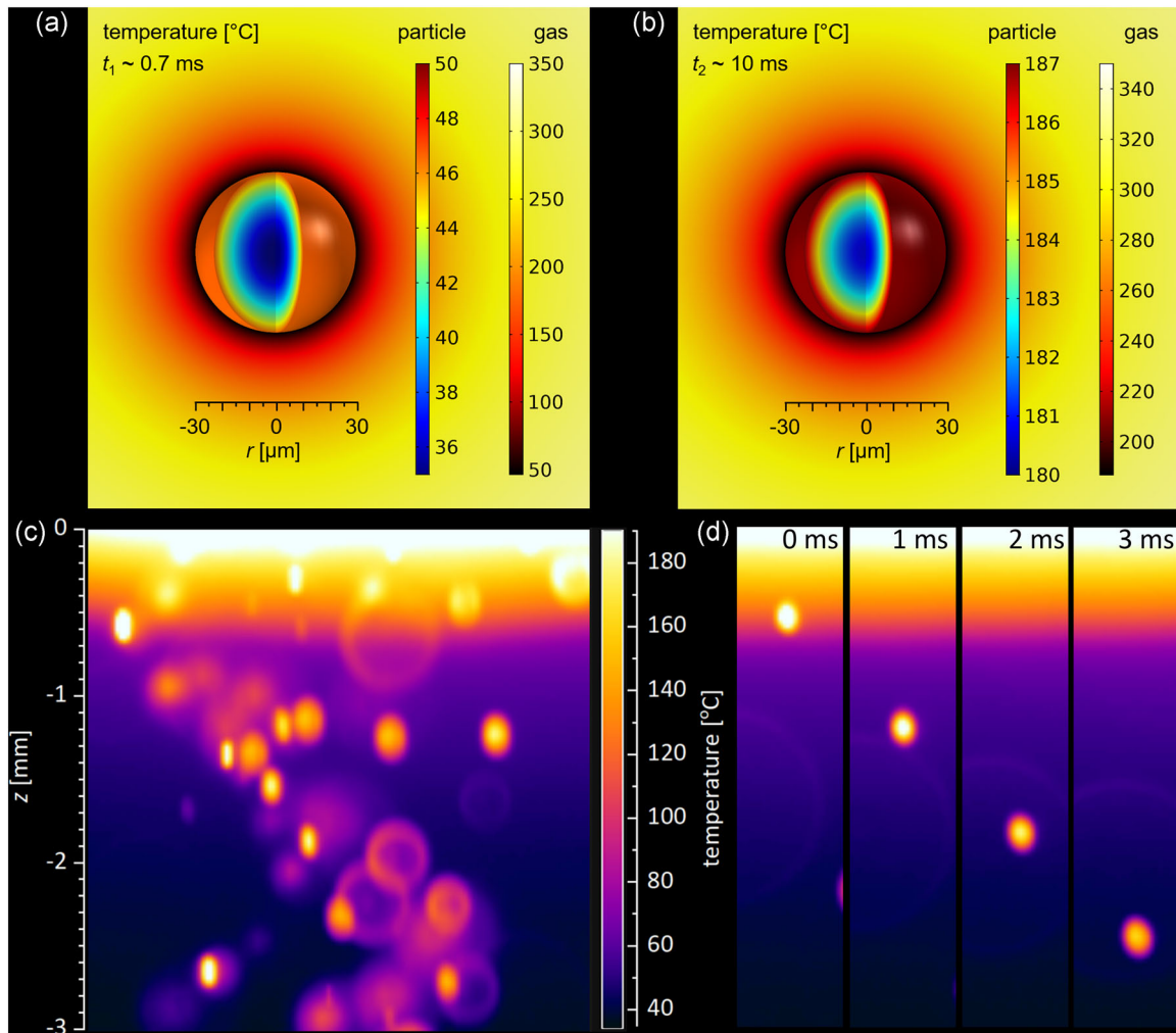
FIGURE 4 Temperature dynamics of particles. Particle and gas temperature obtained from heat-transfer simulations after t_1 = 6.6 \times 10^{-4} s (a) and t_2 = 9.3 \times 10^{-3} s (b), both for a background temperature of 350 ^{\circ}\text{C} ; high-speed IR (infrared) thermography of particles in the effluent at 2 kfps: particle temperature from zoomed area indicated in Figure 3b (c), tracked single-particle movement (d). Note that in (c) and (d) different sizes of particles are caused by IR imaging optics being focused to the axis of the jet. Particles out of focus appear with different size and with incorrect temperatures
