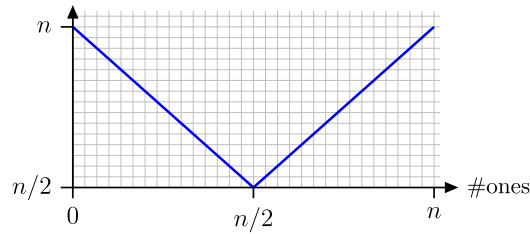
Fig. 1. Sketch of the function TwoMAX.
