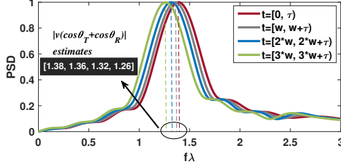
Figure 9: Four adjacent estimates of direction-related parameter |v(\cos\theta_T + \cos\theta_R)| . The estimates are the normalized frequencies corresponding to the peaks of PSD plots.
