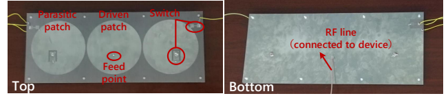
Figure 3: The fabricated antenna system on the receiver side.
