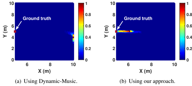
Figure 13: Localization errors of using past (5.1 m) and our (1 m) multipath elimination approaches, when an interfering object locates at point B as shown in Figure 12 (a).
