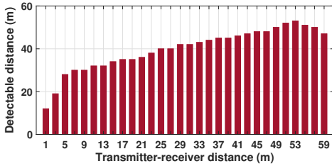
Figure 15: Impact of the transmitter-receiver distance on the detectable distance. WIDEEE can detect a moving object with a distance to the transceiver pair of up to 53 m in an open square.
