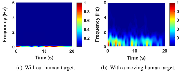
Figure 6: Comparison of the PSD of the received signal when there exists no human target (a) and a moving target (b). The PSD patterns in two scenarios differ significantly.
