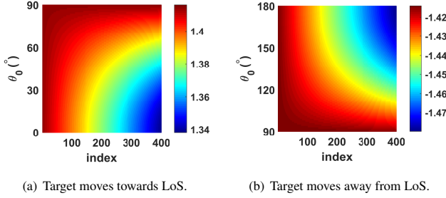
Figure 10: The changing trend of v(\cos\theta_T + \cos\theta_R) estimates at various target moving directions \theta_0 . It can be seen that the changing trend of v(\cos\theta_T + \cos\theta_R) estimates from the 1 st to m^{\text{th}} is always decreasing no matter the target moves towards LoS ( 0^\circ < \theta_0 < 90^\circ ) or moves away from LoS ( 90^\circ < \theta_0 < 180^\circ ).
