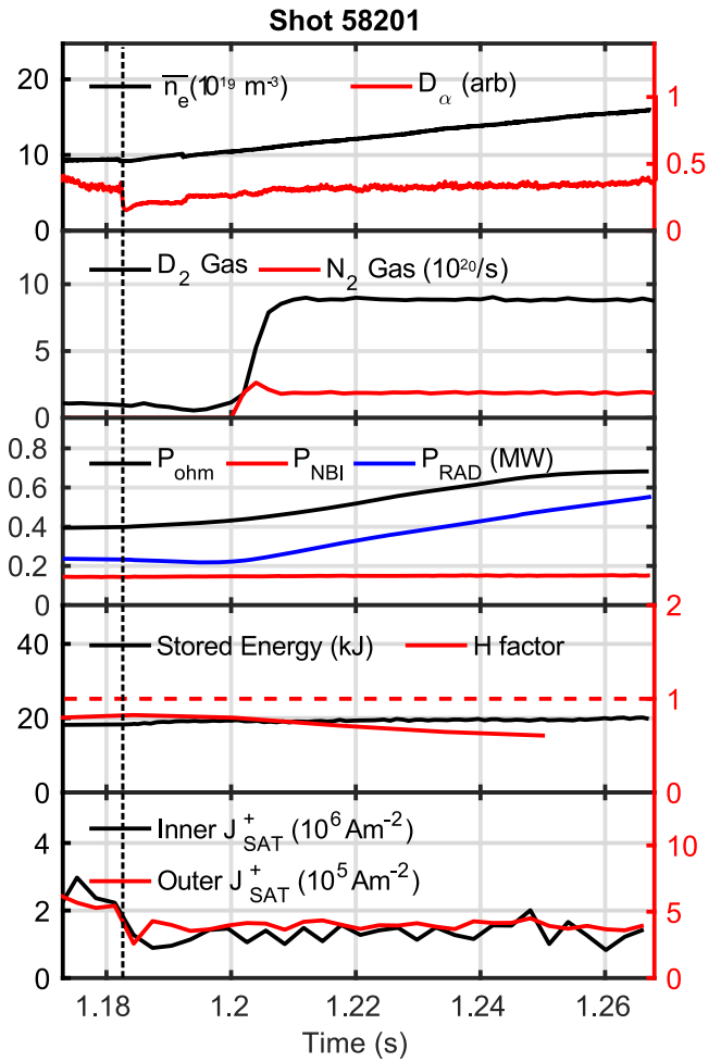
Figure 7. Overview of a typical ELM-free H-mode shot, showing the evolution of the line average density, divertor D_{\alpha} emission, gas fuelling and seeding rates, plasma power sources and sinks, stored energy and confinement quality and the total particle flux to the inner and outer divertors. The L–H transition is indicated by the dashed vertical line.
