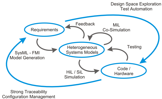
Fig. 1. Connections in the INTO-CPS tool chain
