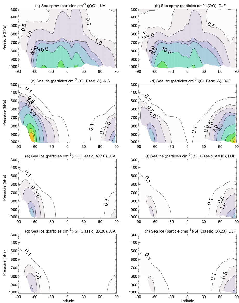
Figure 7. Zonal mean SSA total number concentration ( \text{particles cm}^{-3} ) from the sea spray open ocean in (a) June–July–August (JJA) and (b) December–January–February (DJF) from the OO run. Sea-ice-sourced SSA from the SI_Base_A run shown in (c) and (d), with the SI_Classic_AX10 run result in (e) and (f) and the SI_Classic_BX20 run result in (g) and (h). The plots are based on 1-year (2013) integration. The contour interval is 10 \text{ particles cm}^{-3} when number density is larger than 10 \text{ particles cm}^{-3} .
