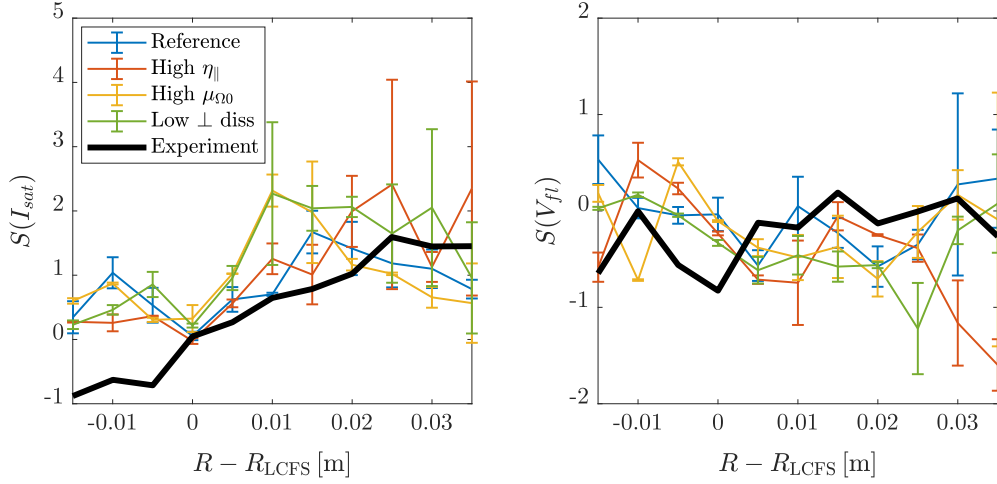
FIG. 5: Skewness of the I_{sat} (left panel) and V_{fl} (right panel) PDFs for the experimental measurements (thick black lines) and the STORM simulations (thin color lines). The error bars represent one standard deviation of the results evaluated at \varphi = 0 and \varphi = \pi/4 .
