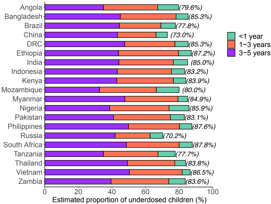
Figure 2. Underdosing prevalence with current WHO treatment guidelines.
