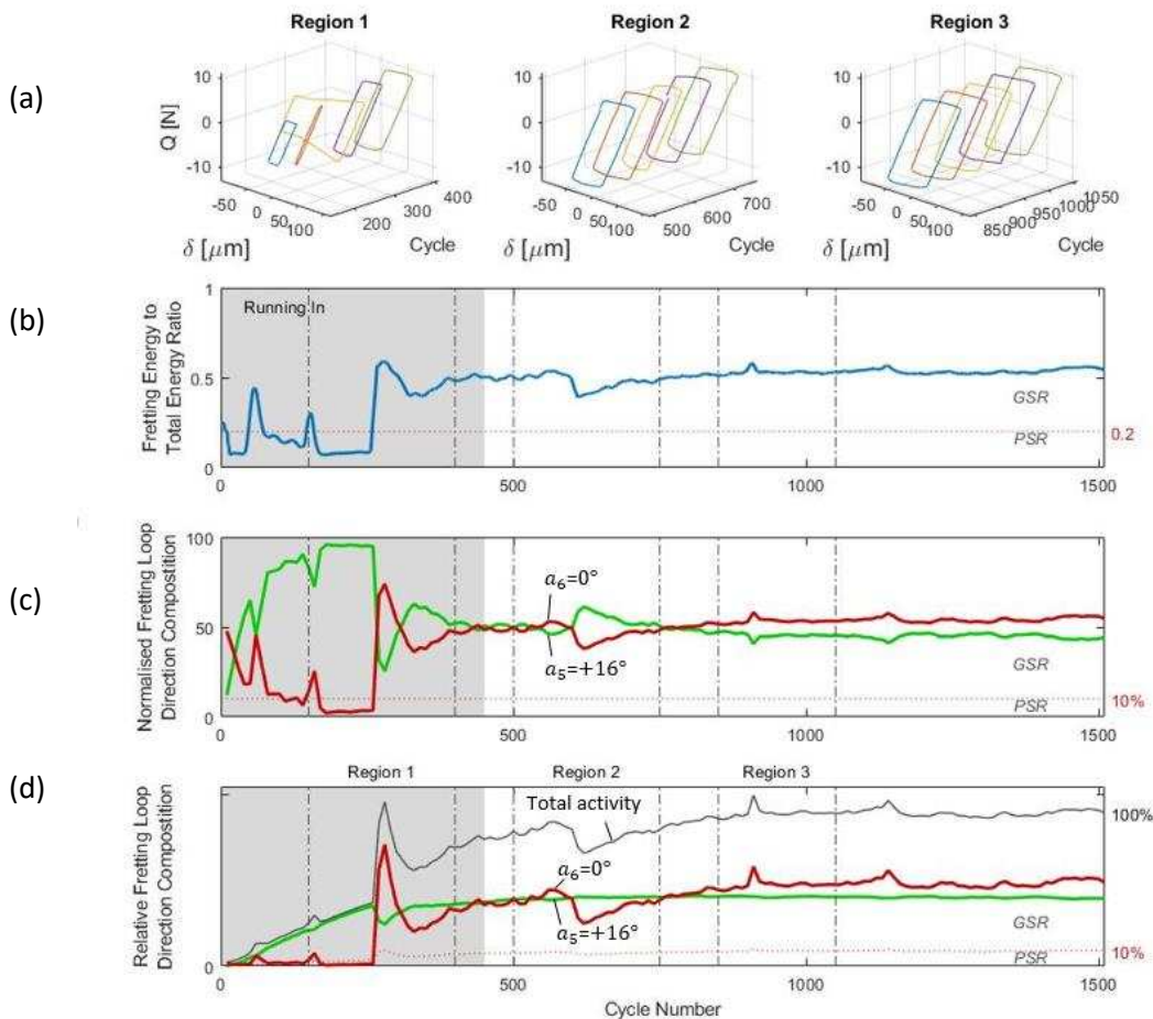
Fig. 7 The \delta^* = \pm 75 \mu m experiment, (a) fretting loops from three regions demonstrating representative fretting behaviour throughout the experiment: (i) Region 1 over transition according to the 10 % a_6 and 0.2 energy ratio thresholds (ii) Region 2 mid test and (iii) Region 3 towards the end of the test, (b) fretting energy to total energy ratio with the 0.2 threshold indicated, (c) normalised percentage fretting loop direction composition with 10 % threshold and, (d) the relative fretting loop direction composition with indicated 'Total activity' indicating 100 % total fretting loop vector magnitude (i.e. the total perimeter of the fretting loop) and threshold at 10% of the total activity. The running in period is indicated as the shaded grey region in b, c and d.
