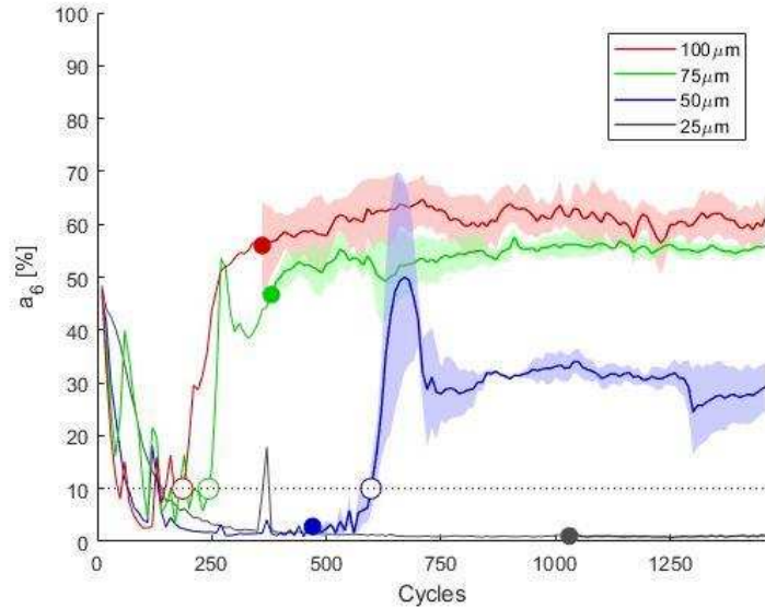
Fig. 9 Mean percentage a_6 composition where the shaded areas represent the standard deviation between the three repeats after the running in period, indicated as after the solid markers. The transition points from PSR to GSR are indicated by white circular markers outlined in the corresponding colour.
