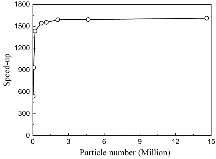
Figure 9: The speed-up of the GPU simulations over the single-core CPU simulations.
