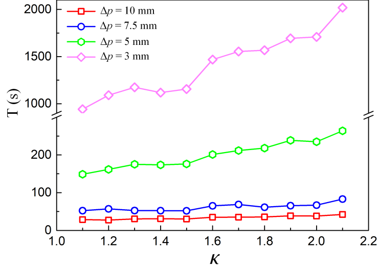
Figure 8: The simulation time used for the simulations.
