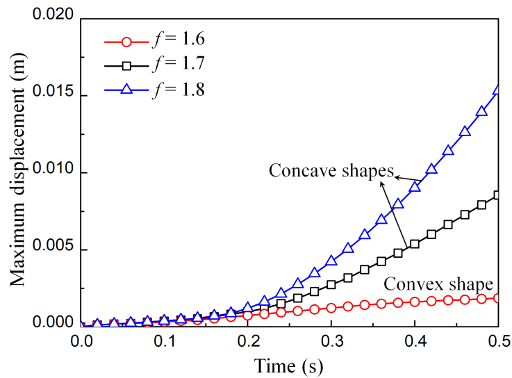
Figure 13: The maximum displacement-time relation under different reduction factor with the hypoplastic model.
