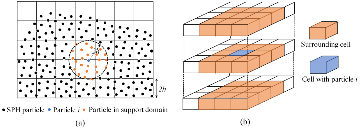
Figure 2: Sketch of the virtual search grid: (a) virtual search grid and support domain in two-dimensions; (b) virtual search grid in three-dimensions.
