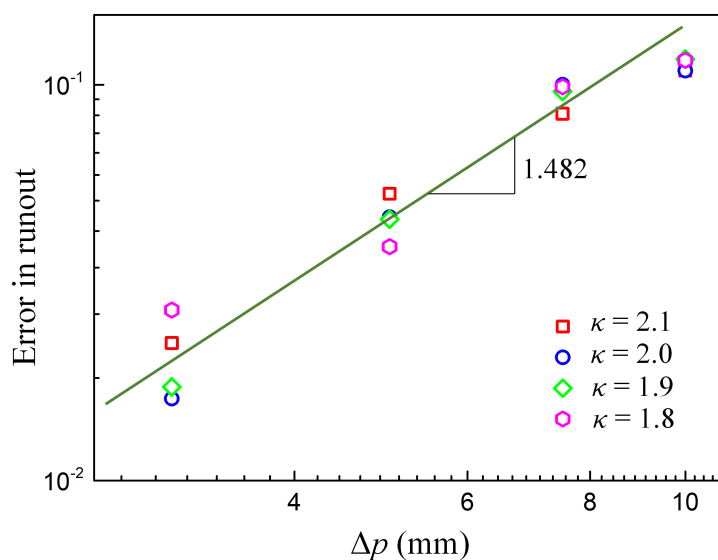
Figure 5: The rate of convergence of the sand collapse simulation.
