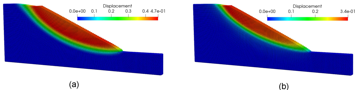
Figure 14: The displacements under reduction factor 1.8 (in meters): (a) Drucker-Prager model, (b) hypoplastic model.
