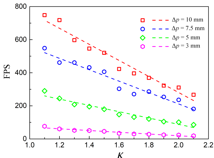
Figure 7: The FPS results from the 44 simulations.
