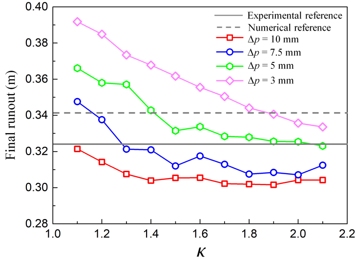
Figure 4: The runout results for all the simulations.
