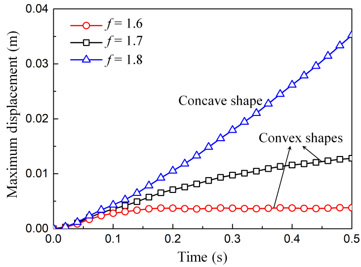
Figure 12: The maximum displacement-time relation under different reduction factor with the Drucker-Prager model.
