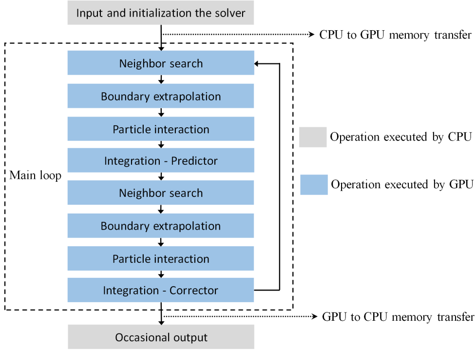
Figure 1: Flowchart of the simulation process in LOQUAT.
