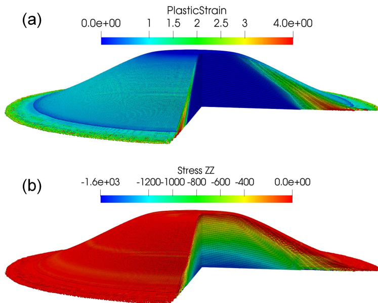
Figure 6: The final profile of the simulation of \Delta p = 1 mm and \kappa = 2.8 with a total particle number of 15.7 million: (a) equivalent plastic strain; (b) vertical stress.
