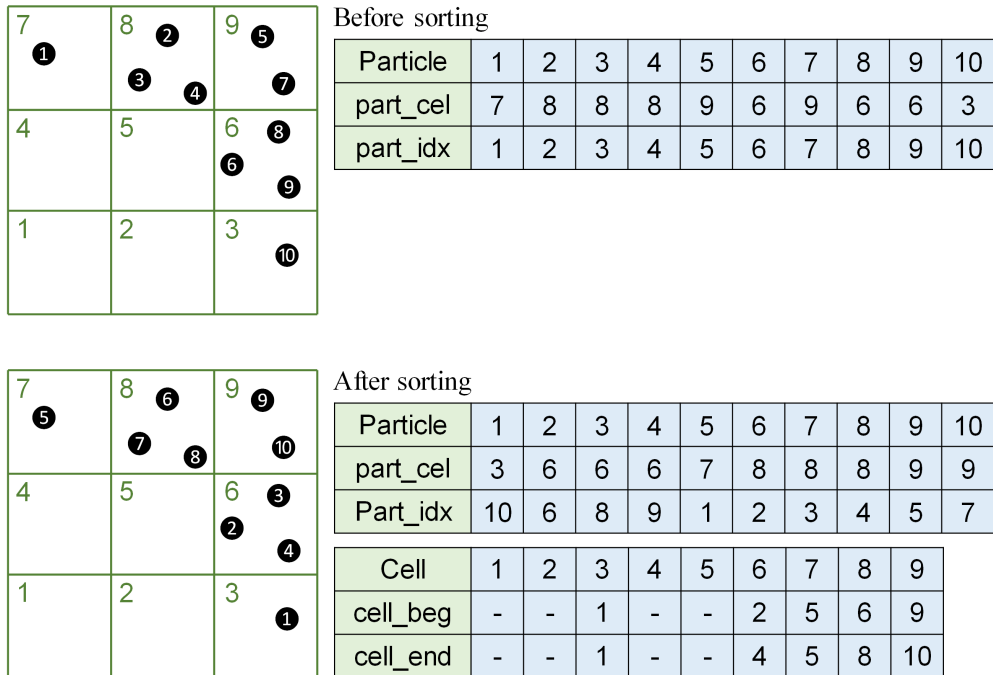
Figure 3: A simple example to show the work flow of the modified linked-list search algorithm.
