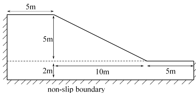
Figure 11: Geometry and boundary conditions of the exemplary slope.
