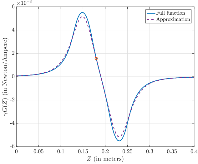
Fig. 3. Function G(Z) (defined in (5)) and its approximation G_{\text{approx}}(Z) in the far field of the magnet (defined in (6)). The circle denotes the value G(\bar{Z}) at the rest position \bar{Z} = 0.18 . The values used for the rest of the parameters are taken from the table found in the appendix of [2].
