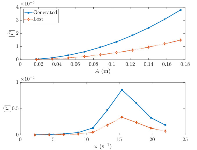
Fig. 6. Variation of the total mean power generated (in Volt×Ampere) against the wavemaker amplitude or frequency. The mean power is calculated from (14) over the duration of one simulation with T = 10\text{s} . Top panel: varied wavemaker amplitude A (in m) with fixed frequency \omega = 8.8\text{s}^{-1} and bottom panel: varied wavemaker frequency \omega (in \text{s}^{-1} ) with fixed amplitude A = 0.0616\text{m} .
