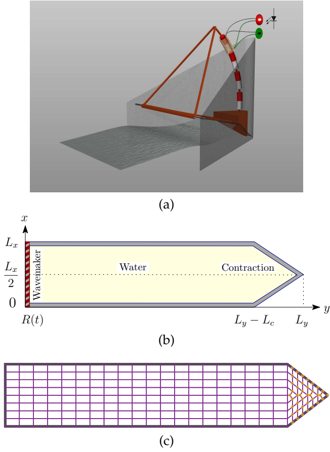
Fig. 2. (a) Sketch of our wave-energy device with its horizontal axel at the contraction entrance, and its three-dimensional buoy in the contraction indicated in orange. The buoy is attached to an induction motor, consisting of magnets on the arc moving through the hollow cylindrical coils indicated in yellow, as well as a green and red LED. (b) Schematic of the wave-energy tank used in the simulations, and (c) the finite-element mesh.
