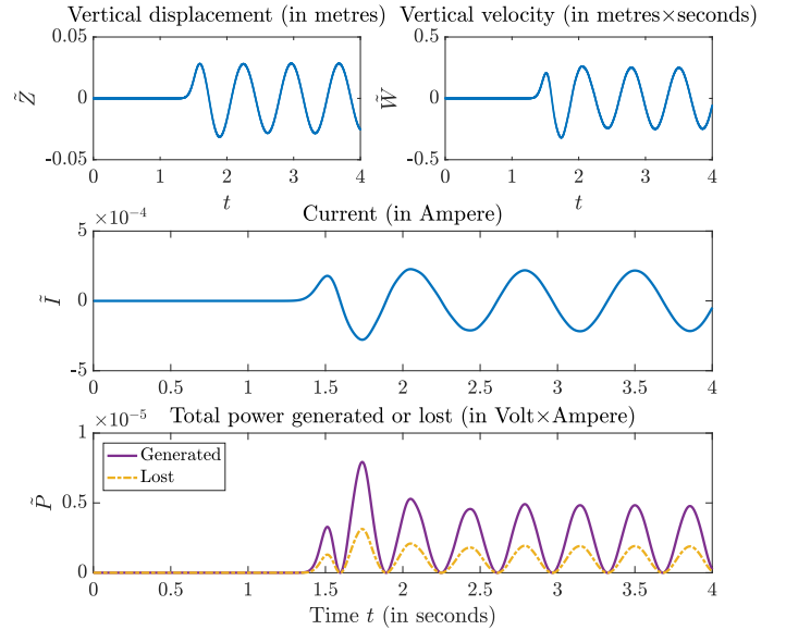
Fig. 5. Output of the numerical simulation demonstrating the response of the wave-energy device to the incoming waves (panels on top row; left: vertical displacement, right: velocity). The energy generated is also shown in terms of current (middle panel) and power (bottom panel). The power output depicted in the bottom panel is divided into two parts: the power output to the LEDs (solid purple line) and the power lost in the electrical circuit (dash-dotted yellow line).
