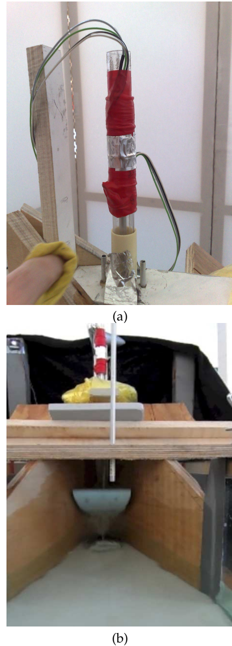
Fig. 1. A proof-of-principle of the scaled wave-energy device is shown: (a) a zoom-in of the electro-magnetic generator showing the hollow tube (covered in red tape) with its coils and the LED; the magnets on top of the buoy-mast move through the coils; and, (b) a view in the contraction with the buoy and a blinking LED light (top left).
