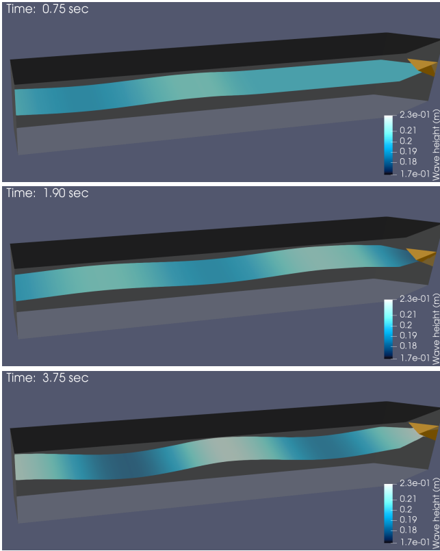
Fig. 4. Snapshots of the numerically computed free surface h(x, y, t) = \bar{H}(x, y) + \eta(x, y, t) (colour denotes height in meters, with initial still water level H_0 = 0.2\text{m} ) as it evolves in the wavetank with V-shaped contraction (times shown on the pictures). The buoy resides in the corner of the contraction and is shown using the orange colour.
