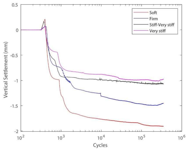
Figure 19. Vertical settlement (Setup C)
