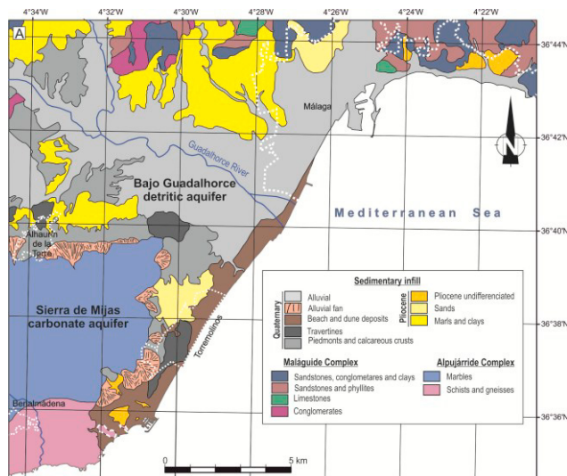
Fig. 2. Geological map of Sierra de Mijas carbonate aquifer and Bajo Guadalhorce detritic aquifer. Modified from 1066 and 1067 MAGNA 50 geological maps 12,13 . White dotted-lines represent the location of the main towns while white dashed-line indicates the sediment/basement boundary.
