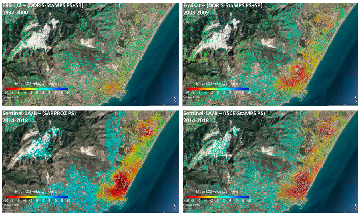
Fig. 4. Mean LOS velocity of the zone 1 (Fig. 3) corresponding to Torremolinos-Benalmádena area.
