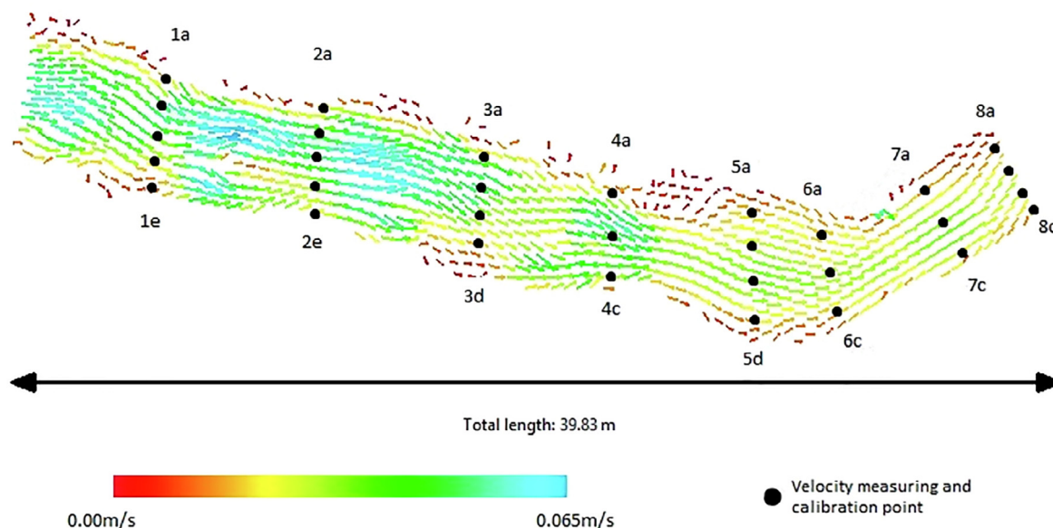
Fig. 2. SRH-2D hydraulic predictions, post-calibration, showing predicted velocity in m/s for an inflow of 0.024 m 3 /s, with in-field velocity measuring point positions.
