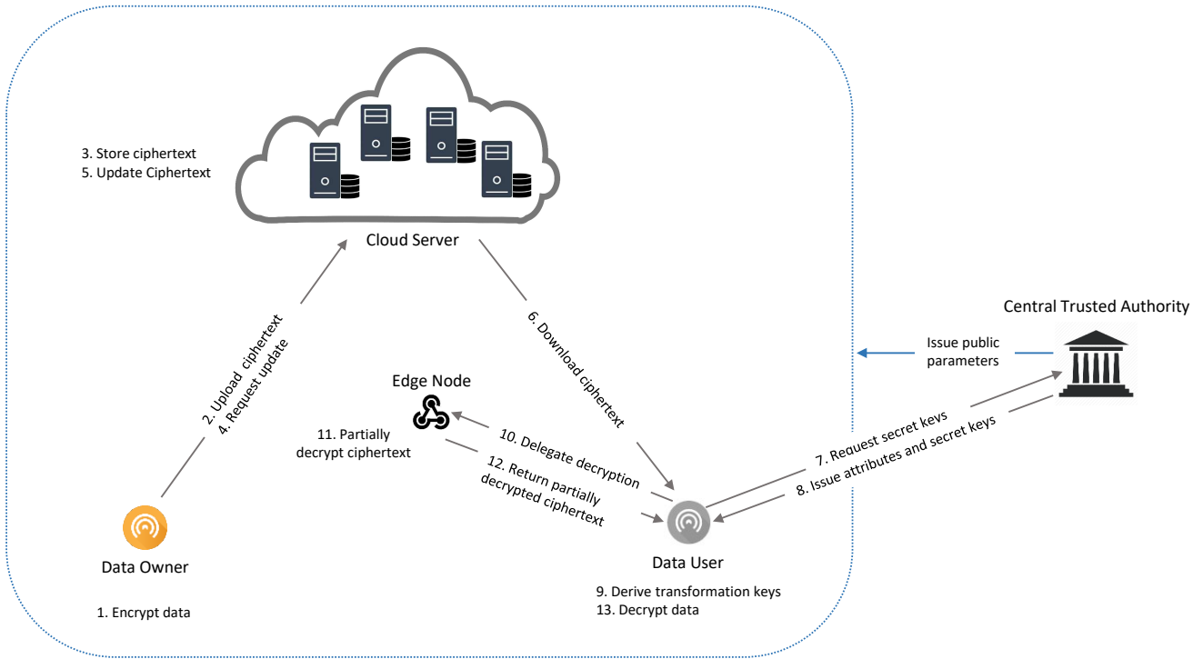
FIGURE 2 CUPS Architecture
