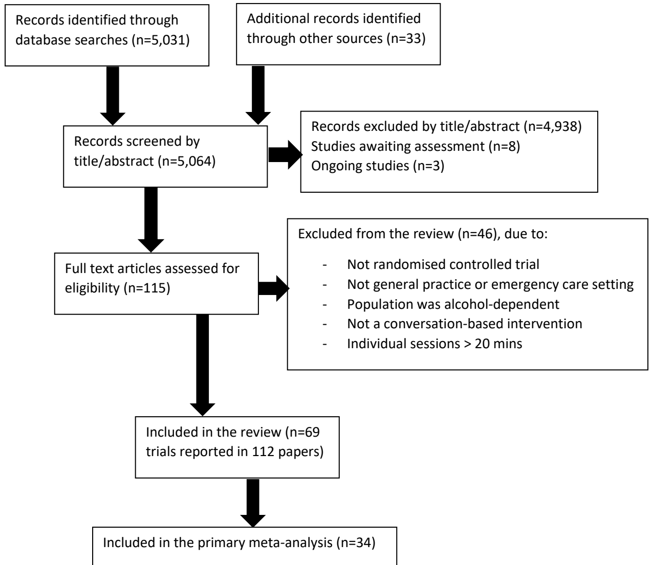
Figure 1: Prisma diagram
