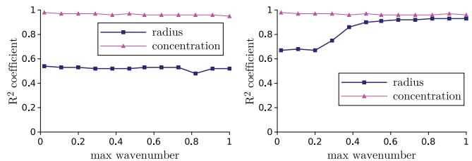
Fig. 5: (Colour online) This figure shows how increasing the maximum wave number does not lead to better predictions of particle radius when measuring \langle u \rangle . That is, for each point (x, y) on the graphs, we limit the incident wave numbers of the training and test set to 0 \leq k \leq x , which results in y = R^2 . On the left (right) we used a model trained on only \langle u \rangle ( \langle u \rangle and \langle u \rangle_2 ).
