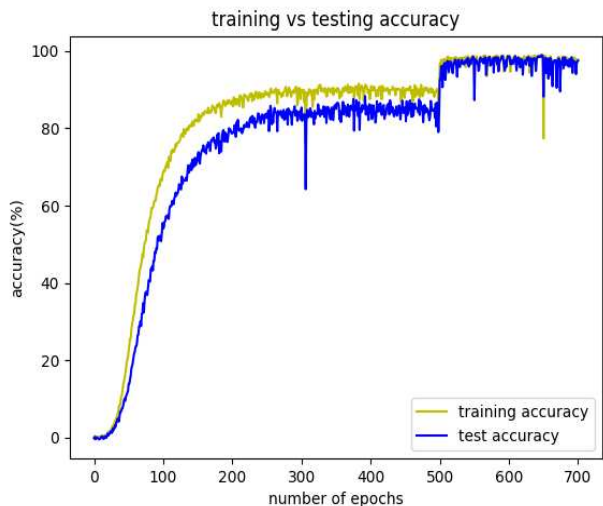
Fig. 5: Training vs Testing accuracy (%) during late fusion model training
