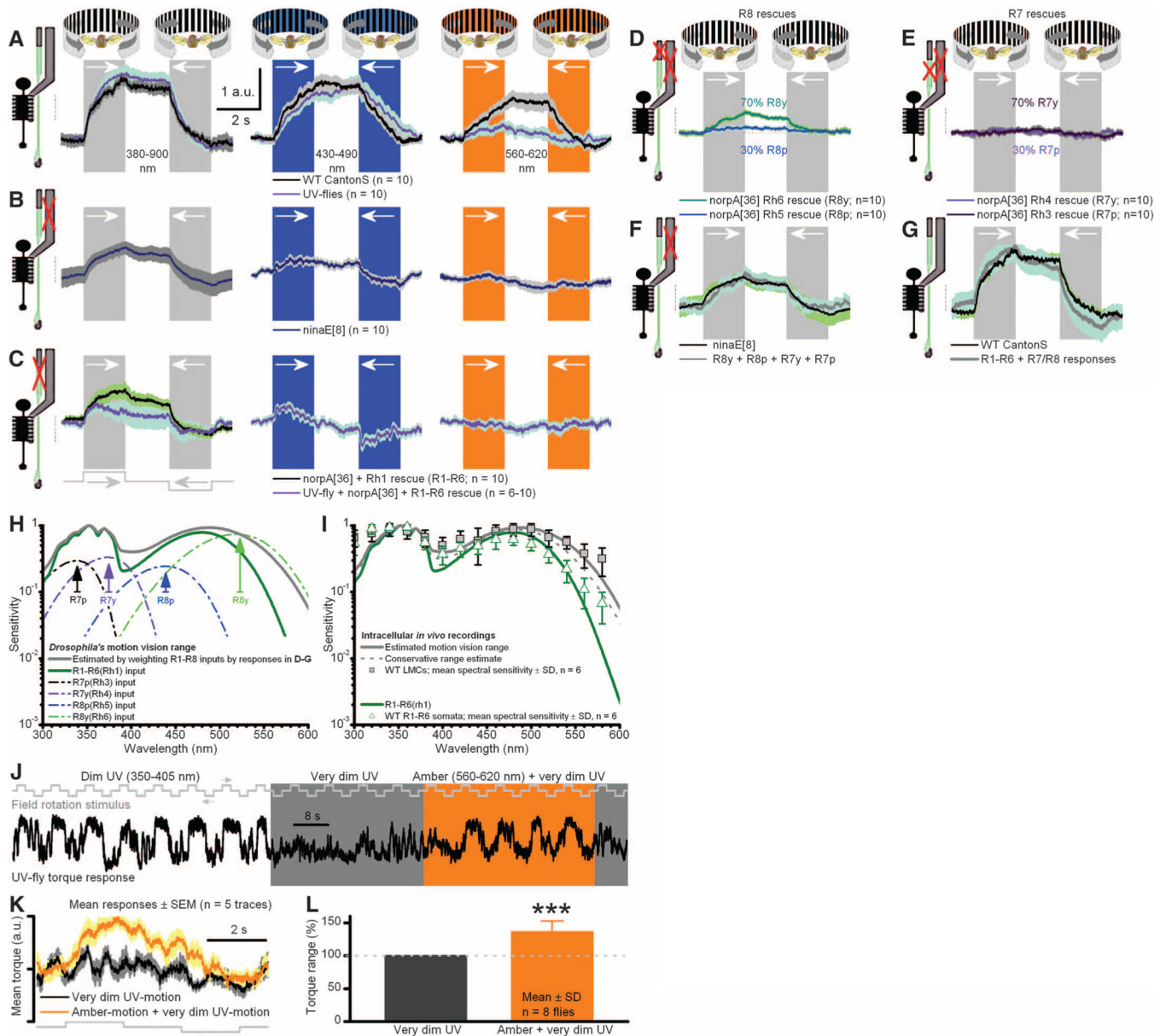
Fig. 4. Signals from R1–R6 and R7/R8 sum to generate optomotor responses. Responses (yaw torque) of tethered flying Drosophila to different color-field rotations (black-white, black-blue, and black-amber) to left and right. (A) Both UV flies (R1–R6s expressing Rh3-opsin) and WT respond to broad spectral range of motions. a.u., arbitrary unit. (B) Mutant ninaE 8 -flies, having light-insensitive R1–R6 photoreceptors (Fig. 3G; motion pathway) but normal R7/R8 photo-receptors, react to an equally broad spectral range of motions as in (A) , but with weaker responses. (C) norpA 36 flies, having R1–R6 photoreceptors rescued with Rh1 or Rh3 opsins, react to broad spectral range of motions but with weaker and faster responses than in (A) . (D) Rescuing light sensitivity only in R8y or R8p photo-receptors enables visual motion perception. (E) Rescuing light sensitivity only in R7y or R7p photoreceptors enables weaker motion perception (fig. S11B). (F) Responses of norpA 36 flies with rescued light
