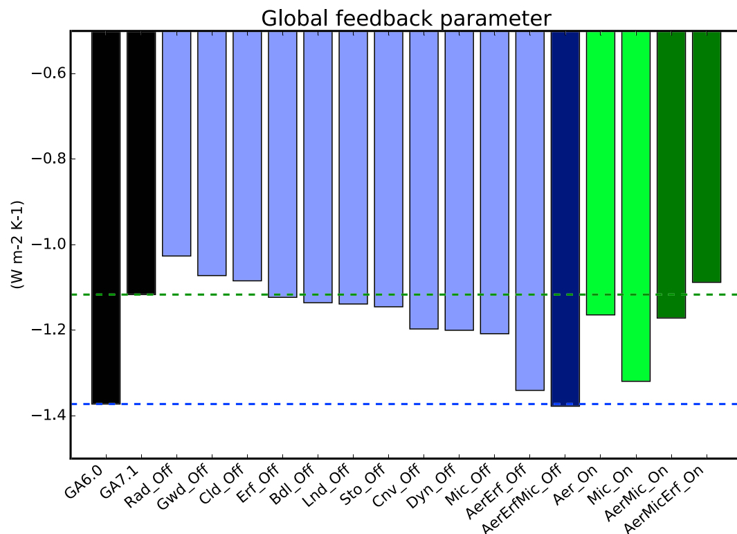
Figure 1. Global-mean feedback parameter. The two control experiments, GA6.0 and GA7.1, are shown in black. The blue bars correspond to the Off experiments, and the green bars to the On experiments. Each color has two shades: the light shade shows experiments where only one package is changed, and the dark shade when more than one package is changed. Two horizontal lines are shown that serve as the target control experiments: blue for the target of the Off experiments (GA6.0), and green for the target of the On experiments (GA7.1).
