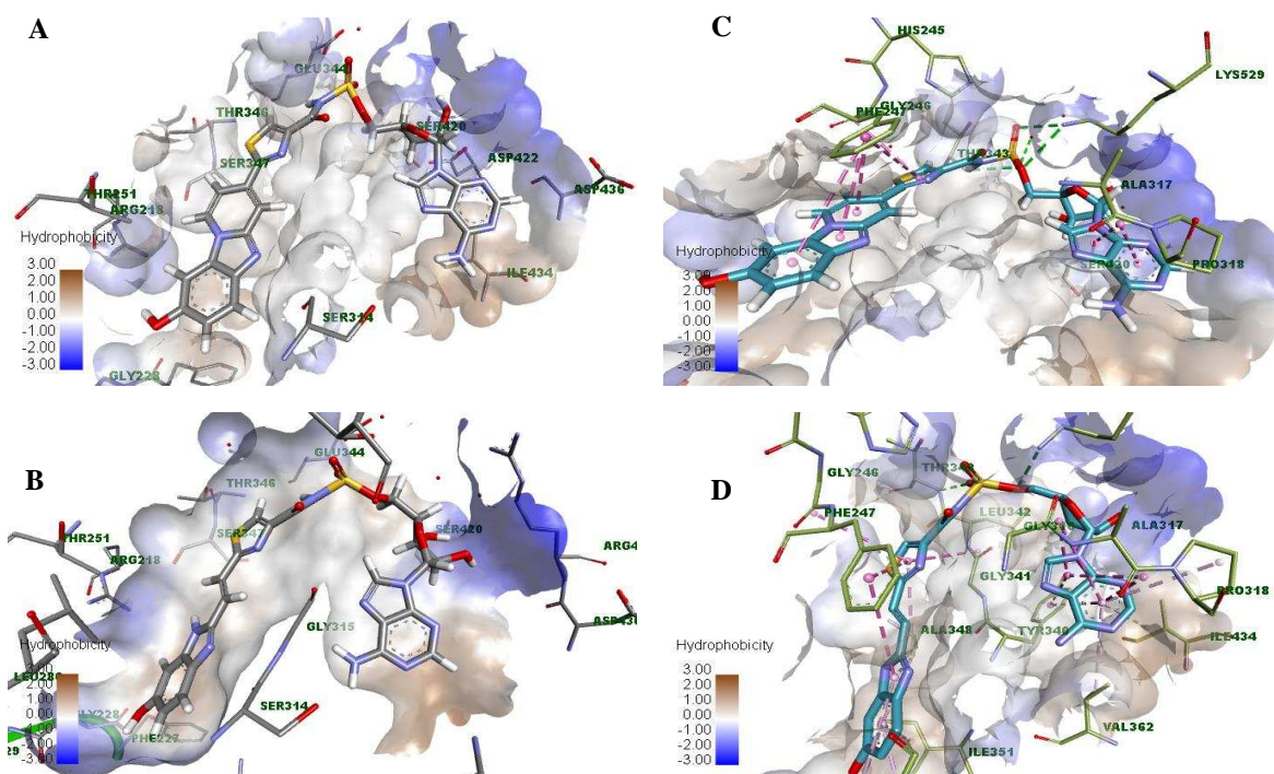
Fig. 3. - A and B - Pose prediction for PBIiLH 2 and BliiLH 2 in PpyLuc pocket; C and D - PBIiLH 2 and BliiLH 2 with predicted interactions; Colour code: Pink – Hydrophobic interactions; Green – hydrogen bonds
