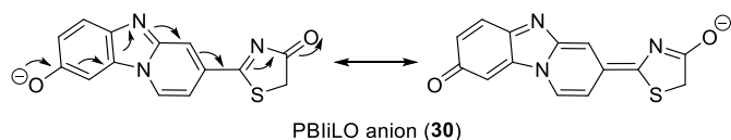
Figure 6. Potential resonance forms of light emitting PBiLO ( 30 ) in its deprotonated form.
