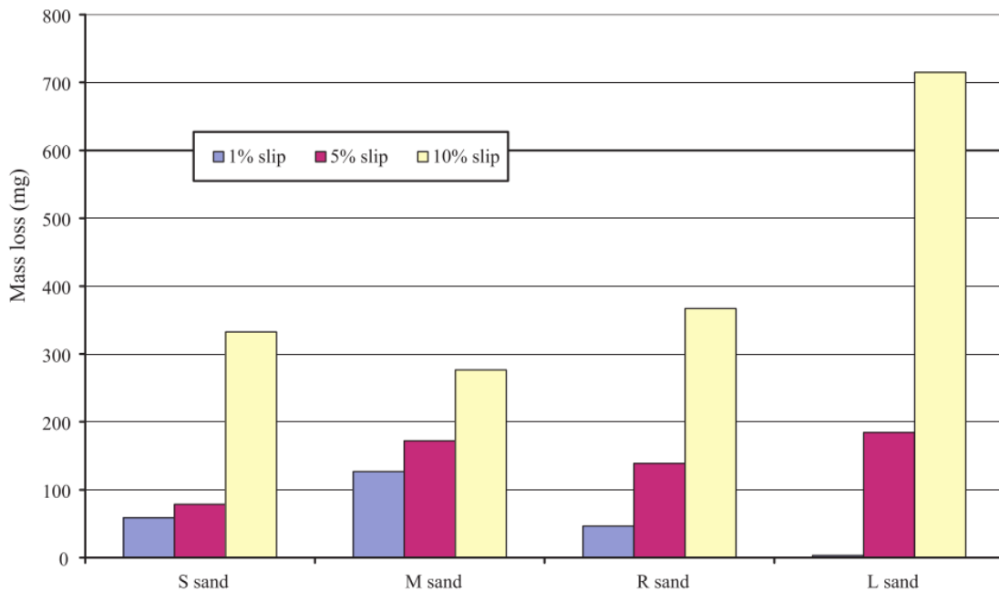
Figure 10 – Mass Loss due to Wear at a range of particle sizes and slip rates. 17
