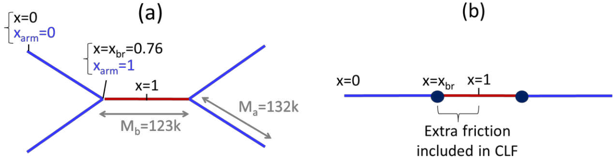
Figure 7: (a) H-polymer molecular coordinate systems. The first one, from the end of the branches, x_{arm}=0 , to the branch point, x_{arm}=1 , is used for determining the relaxation time of the molecular segments around the arms. The second one, from the end of the branches, x=0 , to the middle of the backbone, x=1 , is used to determine the relaxation time of the (inner) backbone. (b) At time longer than the relaxation time of the branches, these last ones are seen as extra friction points along the backbone of the H-polymer.
