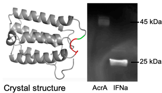
Figure 3. N-glycosylation of IFN- \alpha 2b in E. coli (left: crystal structure. GVGVT amino acid sequence was changed to EVNVT. In PDB, 1ITF GVGVT is at position 102–106. The T corresponds to the O-linked glycosylation site as residue T106 (The 102GVGV105 is marked in red and T106 in green); right: lectin peroxidase blot with AcrA control.
