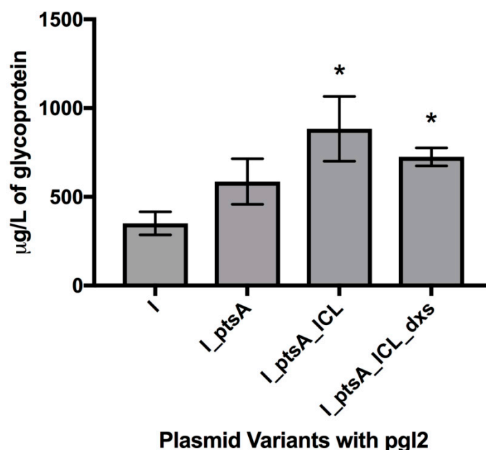
Figure 5. Average \mu\text{g} glycoprotein per litre of cell culture expressing IFN- \alpha 2b along with the metabolic engineering genes and the pgl2 machinery. CLM24 pEC ( IFN- \alpha 2b ) pACYC ( pgl2 ) is included for a comparative control. Quantity was calculated through measuring the density of glycosylated bands of IFN- \alpha 2b compared to a loading control of 0.5 \mu\text{g} of purified AcrA. “I” denotes IFN- \alpha 2b expression and asterisks (*) above the bars indicate strains of significant difference from the control (Unpaired t-test with Welch’s correction, n = 3 ; P < 0.05 ).
