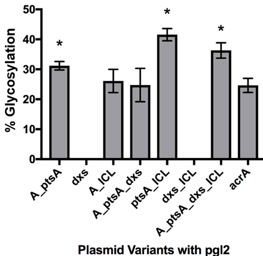
Figure 2. Glycosylation efficiency of the strains expressing acrA , the metabolic engineering genes and the p gl2 machinery. Cells without metabolic engineering of central carbon metabolism, CLM24 pEC(acrA) pACYC(p gl2 ), was included for a comparative control. Efficiency calculated through measuring the density of aglycosylated and glycosylated bands of AcrA. “A” denotes acrA expression and asterisks (*) above the bars indicate strains of significant difference from the control (Unpaired t-test with Welch’s correction, n = 3; P < 0.05). AcrA is the control strain comprising of the target protein gene ( acrA ) and glycosylation machinery contained in the p gl2 plasmid without any additional metabolic engineering elements.
