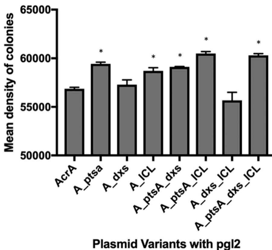
Figure 1. Mean density measurements for colonies in positive control strain ( AcrA is acrA with pgl2 ) and engineered strains. Error bars represent the standard deviation of 55 colonies. Asterisks (*) above the bars indicate strains of significant difference from the control (Unpaired t-test with Welch's correction, n = 3 ; P < 0.05 ).
