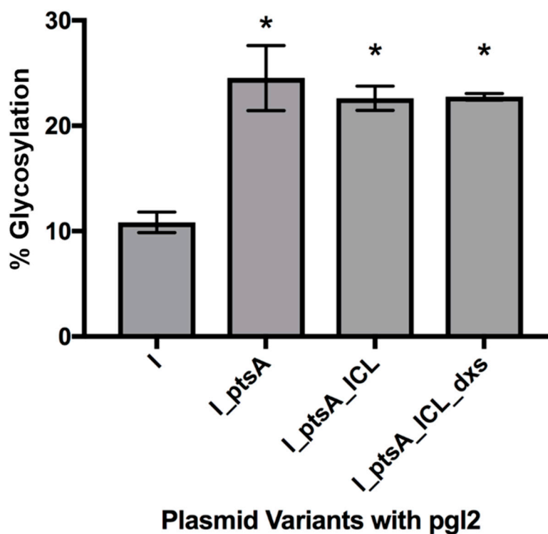
Figure 4. Glycosylation efficiency of the strains expressing IFN- \alpha 2b, the metabolic engineering genes and the pgl2 machinery. CLM24 pEC (IFN- \alpha 2b) pACYC (pgl2) is included for a comparative control. Efficiency was calculated through measuring the density of glycosylated and glycosylated bands of IFN- \alpha 2b. “I” denotes IFN- \alpha 2b expression and asterisks (*) above the bars indicate strains of significant difference from the control (Unpaired t-test with Welch’s correction, n = 3; P < 0.05).
