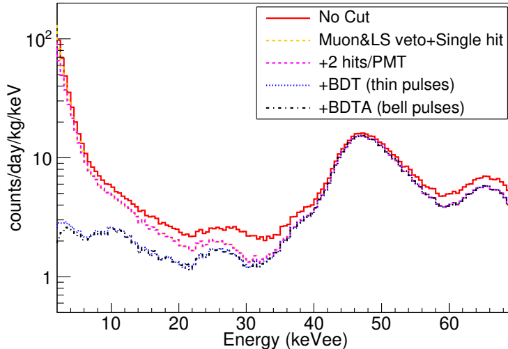
Figure 2. Staged event selection versus energy. The low-energy spectrum between 2 and 70 keVee is displayed with the progression of application of the selection criteria. The selection efficiency is uncorrected here.
