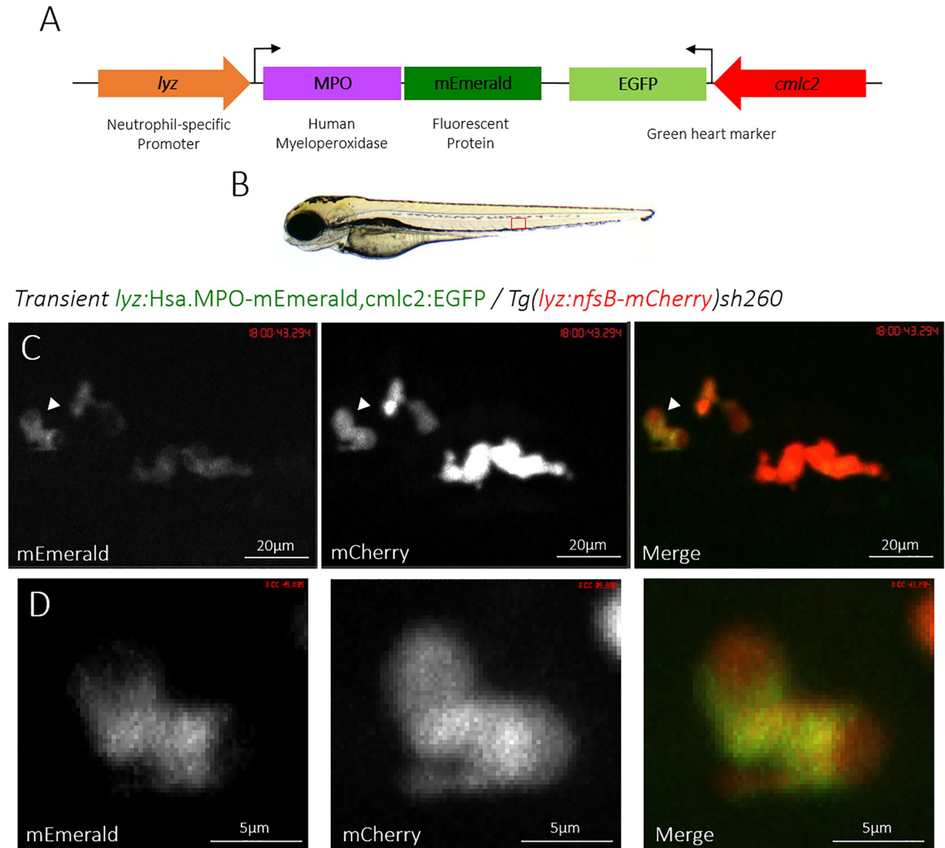
Fig 1. Transient expression of the lyz :MPO-mEmerald cmlc2 :EGFP construct, which includes the neutrophil-specific promoter ( lyz ), the MPO gene with a C-terminal fluorescent tag (MPO-mEmerald) and a green heart marker to aid optimisation of transgenesis ( cmlc2 :EGFP). B) A zebrafish larva at 3 days post fertilisation (dpf), with the caudal haematopoietic tissue (CHT) indicated by the red box. C) The CHT of a double-transgenic Transient lyz :MPO-mEmerald, cmlc2 :EGFP; Tg(lyz:nfsB-mCherry)sh260 larva with a population of neutrophils expressing both mEmerald and mCherry. The white arrowhead indicates the neutrophil enlarged below. D) Enlarged view of a neutrophil expressing mEmerald and mCherry.
