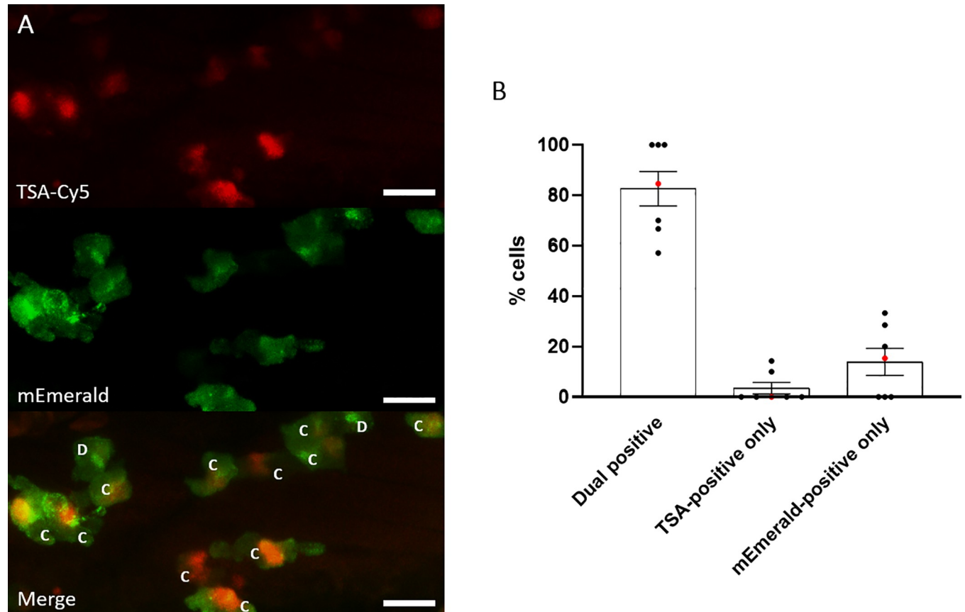
Fig 3. Most MPO-mEmerald-positive neutrophils are TSA-positive. A) Confocal photomicrographs shown as maximum intensity projections of lyz :MPO-mEmerald larvae fixed at 3 dpf and chemically stained with TSA-Cy5. Dual-positive (C) and mEmerald-positive only (D) cells are indicated; scale bar 10 \mu m. B) Quantification of dual positive, TSA-positive only and mEmerald-positive only cells observed in lyz :MPO-mEmerald larvae fixed at 3 dpf and chemically stained with TSA-Cy5. Red points indicate larva shown in A).
