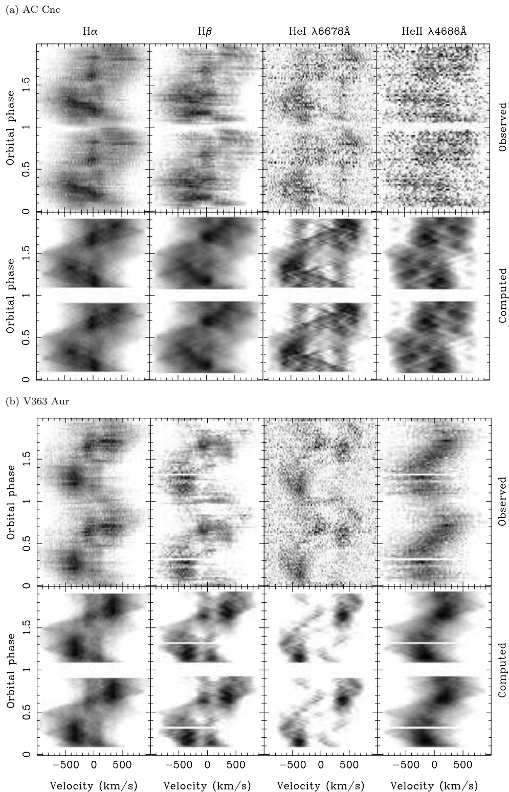
Figure 3. (a) Trailed spectra of AC Cnc (upper panel) and data computed from the Doppler maps (lower panel). (b) Trailed spectra of V363 Aur (upper panel) and data computed from the Doppler maps (lower panel). A comparison of the upper and lower panels gives some indication of the quality of the fit. The gaps in the computed data correspond to eclipse spectra (selected using the light curves of Fig. 2), which have been omitted from the fit as Doppler tomography cannot properly account for these phases. Note that the data have been folded to show more than one binary cycle.
