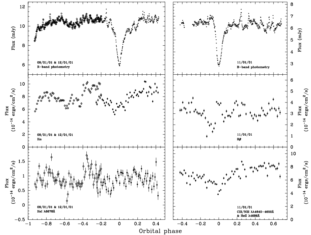
Figure 2. Light curves of (a) AC Cnc and (b) V363 Aur. Top panels: R - and B -band JKT light curves. Middle and bottom panels: emission-line light curves of H\alpha , H\beta , C III/N III \lambda\lambda 4640\text{--}4650 + He II \lambda 4686 and He I \lambda 6678 . The R -band V363 Aur data are from two nights; open circles represent data from 2001 January 12 and closed circles represent data from 2001 January 9. Note that the two nights of data are split by orbital phase, as well as by night of observation.
