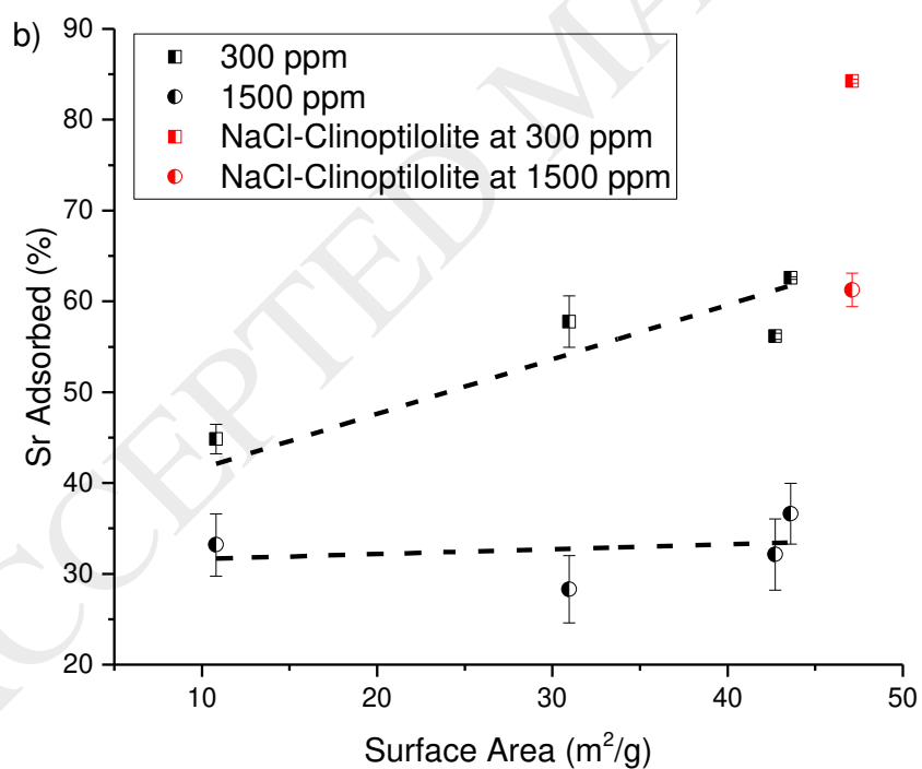
Figure 10: Adsorption percent versus specific surface area for the different mill fractions, as well as salt activated clinoptilolite at two different initial salt concentrations; a) \text{Cs}^+ and b) \text{Sr}^{2+} . Dashed lines represent linear fits to the milled fractions.
