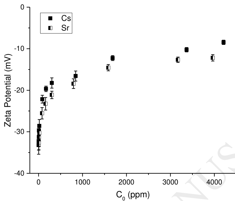
Figure 4: Zeta potential of natural clinoptilolite at neutral pH with different concentrations of Cs + and Sr 2+ ions.
