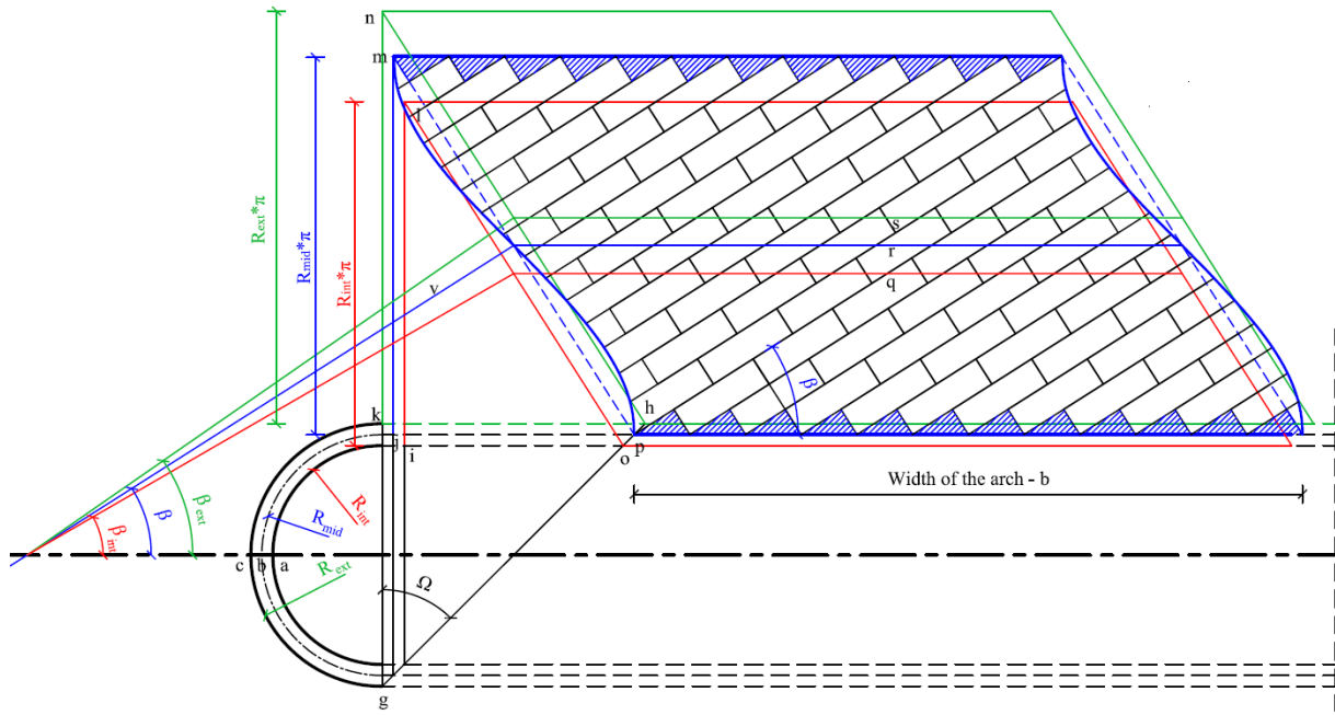
Figure 7 – Charles Fox's drawing type design method to construct the developed surfaces.
