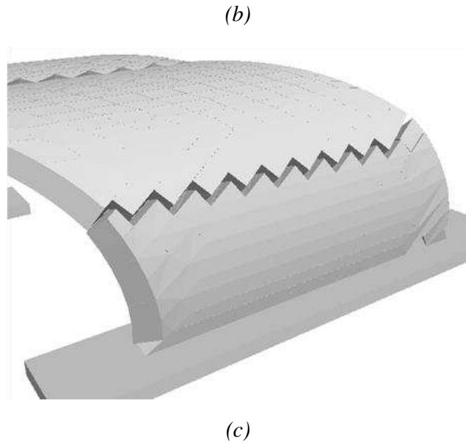
Figure 20 – Failure mode of a helicoidal skew arch (angle of skew 45°)
