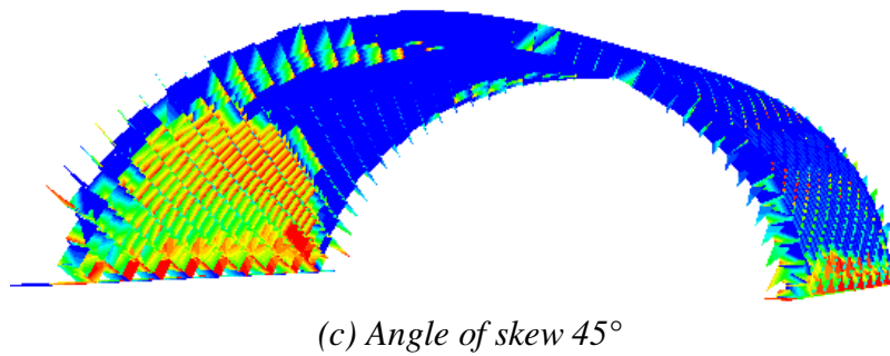
Figure 30 – Shear / normal subcontact stress ratio in case of helicoidal method
