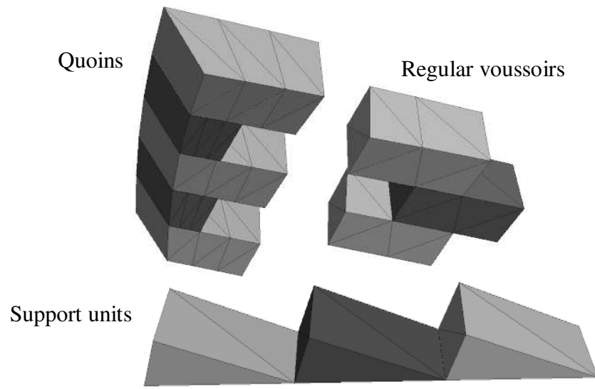
Figure 10 – Elements of the helicoidal skew arch: quoins (top left), normal units (top right), support elements (bottom)
