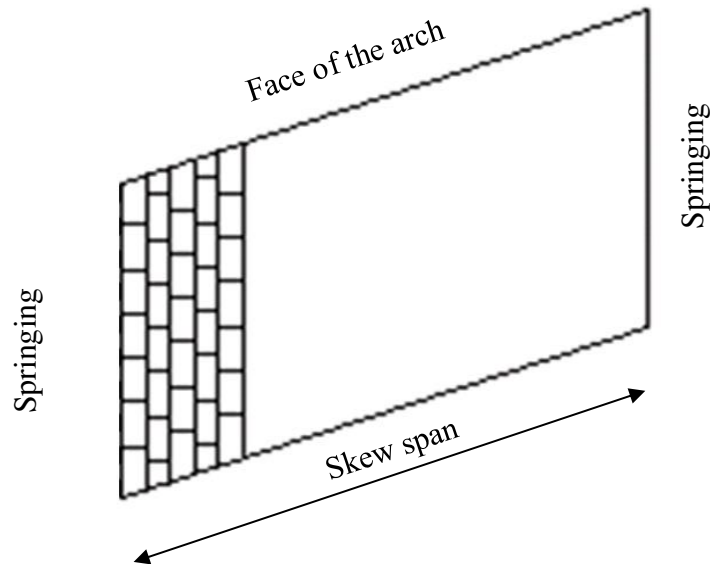
Figure 4 – Plan view of skew arch constructed according to the false method
