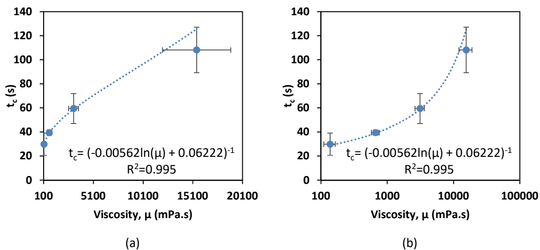
Fig. 8. Time taken for coating completion ( t_c ) plotted as a function of coating liquid viscosity a) normal viscosity and b) log viscosity. Error bars represent standard deviation.
