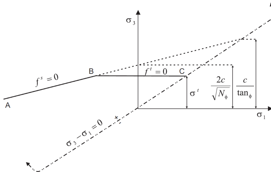
Figure 3: Mohr-Coulomb failure criterion used for plastic block behavior (Itasca 2018)
