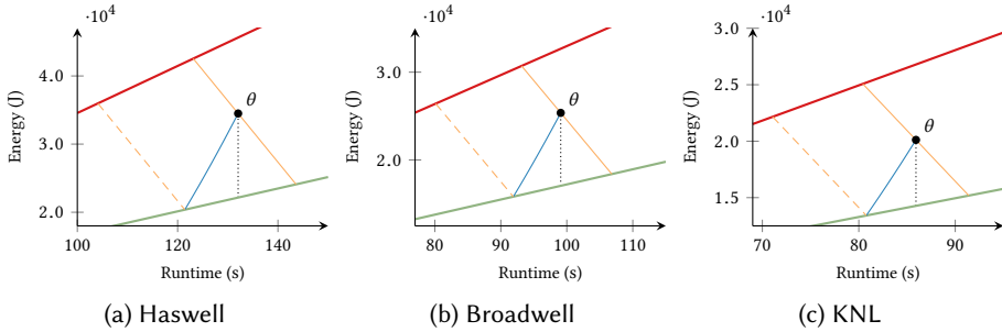
Fig. 5. EDS POSE Models for miniMD using MPI
