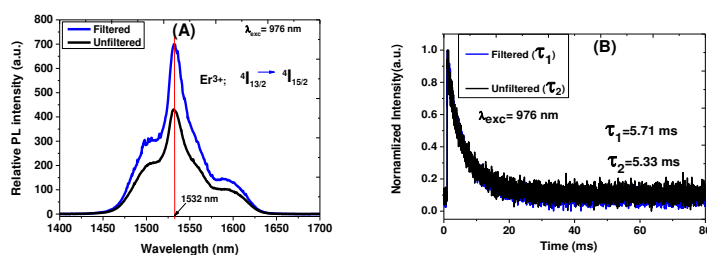
Fig. 1: A) PL spectra of Er ions intra-4f atomic transition {}^4I_{13/2} \rightarrow {}^4I_{15/2} in unfiltered and filter polymer nanocomposite thin films at room temperature under 976 nm excitation source; (B) Corresponding lifetime transients.
