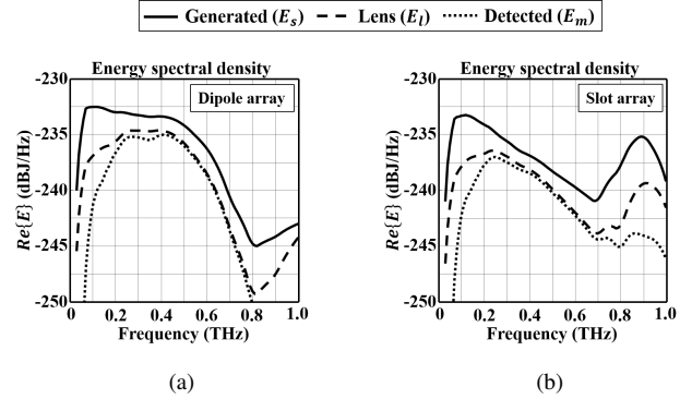
Figure 10. Simulated energy spectral density of the PCCA: a) dipole array and b) slot array, respectively. The plots show the energy spectral densities generated by the arrays E_s (solid lines); the energy spectral densities radiated by the dielectric lens fed by the arrays E_l (dashed line); and the detected energy spectral densities E_m (dotted line).
