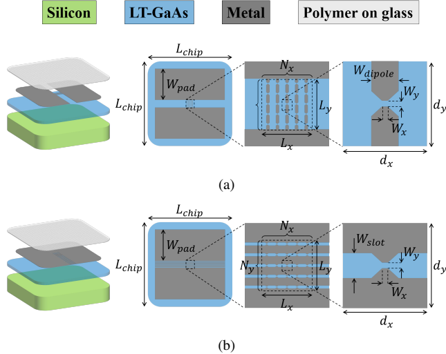
Figure 3. Structures of the PCCA designs. The blue slab represents photoconductive material chip; the green thick slab depicts the silicon lens; the array metallizations are depicted in grey; whereas the micro-lenses array is represented by the light gray slab. a) Dipole based structure, b) slot based structure. The arrays are composed by N_x = N_y = 5 square cells, cells size d_x = d_y = 100 \mu\text{m} , array length L_x = L_y = 0.5 mm, bias pad width W_{pad} = 2.25 mm, and overall chip dimension L_{chip} = 6 mm. Dipole width W_{dipole} = 20 \mu\text{m} , slot width W_{slot} = 30 \mu\text{m} , and gap size W_x = W_y = 7.5 \mu\text{m} .
