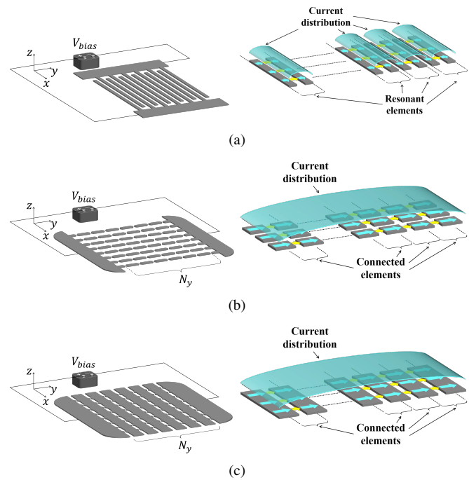
Figure 2. Biasing networks and relevant current distributions of photoconductive interdigitated array and connected array: a) interdigitated based structure, b) dipole based connected structure, and c) slot based connected structure. The yellow arrows represent the impressed currents at multiple periodic locations, the light blue arrows represent the induced current on the array elements. The shaded light blue surfaces depict the current amplitude distribution on the array structures.
