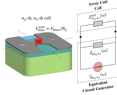
Figure 15. Array unit cell, and Norton equivalent circuit representation.
