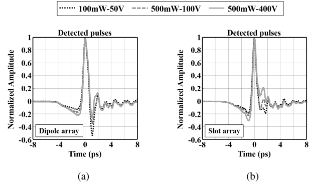
Figure 13. Normalized radiated pulses measured by the EO crystal for different laser power excitations and bias voltages: a) Dipole array, b) Slot array.
