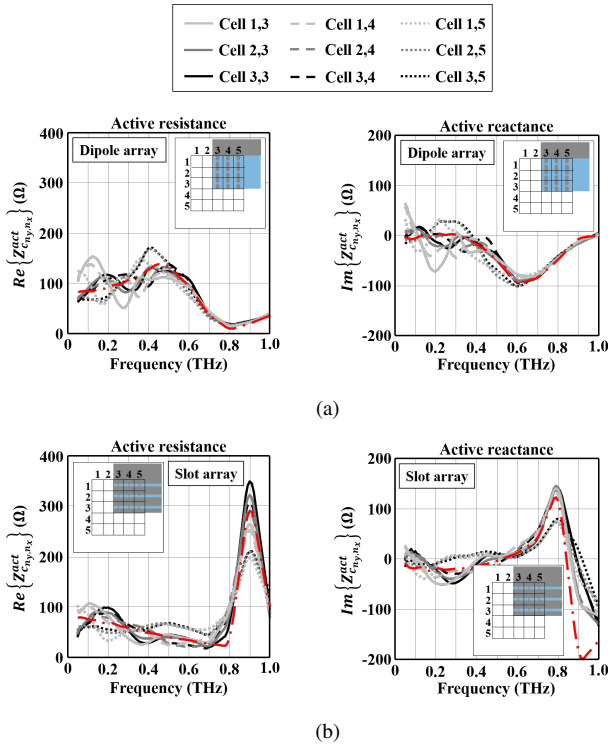
Figure 7. Active impedance of the array cells: a) dipole based design; b) slot based design. Because of the symmetrical excitation of the array elements, only the active impedances of the cells in a quarter of the arrays are shown. The red dash-dotted lines refer to the active resistances and reactances of the unit cell in an infinite connected array configuration.
