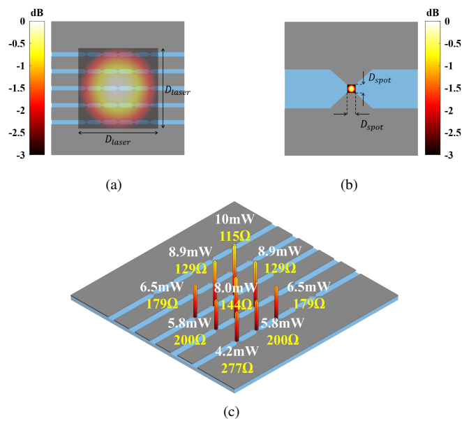
Figure 4. Laser power excitation of the array: a) normalized laser beam distribution on the array area before the focusing of the micro-lenses array; b) normalized laser beam distribution focused by the micro-lens array on each cell gap; c) laser power excitation (white text) and relevant generator impedances (yellow text) on the gaps of the array cells, assuming the maximum available laser power. Because of the spatial symmetry of the laser beam only a quarter of the array excitation is shown, in the picture the slot based array is depicted. The same laser excitation is applied to the dipole based design.
