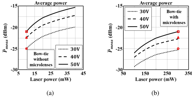
Figure 14. Measured average power versus laser power excitations for different applied bias voltage of the bow-tie antennas for the retrieval of the laser spot focused by the micro-lenses array: a) Bow-tie without micro-lenses array; b) Bow-tie with micro-lenses array. The three red markers in the figures identify the working points where the two devices radiate the same amount of average power.
