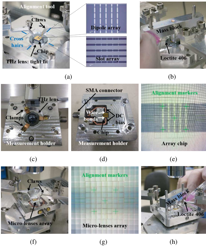
Figure 5. Assembly procedure: a) THz lens and array chip mounted into the auxiliary alignment tool; b) Mass block placed on top of the chip during the glueing to prevent the creation of an air gap between the THz lens and the array chip; c) Front view of the experiment holder with the THz lens and array chip assembly mounted in it. This assembly is kept in place with three clamps; d) Back view of the experiment holder with the THz lens and array chip assembly mounted in it. The DC bias lines are connected to the chip with wire bonds; e) Microscope on-screen markers for the center and the four corners gap elements of the array; f) Alignment of the micro-lenses array with the antenna array; g) Microscope on-screen markers to align the micro-lenses array with the antenna array; h) Mass block placed on top of the micro-lenses array during the glueing to assure that no glue goes under the micro-lenses array.
