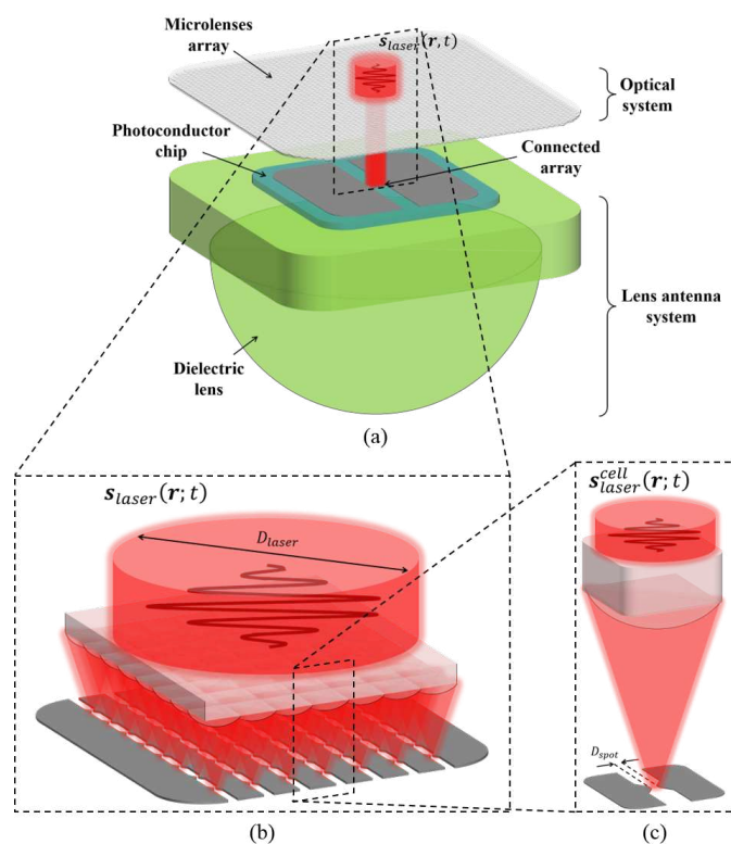
Figure 1. Structure of the photoconductive connected array: a) general view of the system structure, b) view of the connected array and its excitation optical network, and c) view of the cell excitation.
