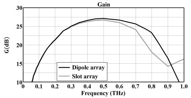
Figure 8. Simulated gain of the array designs. The evaluation of the gain takes into account the front-to-back losses, the dielectric losses of the silicon, and the reflection losses at the lens interface including the effect of the matching layer.
