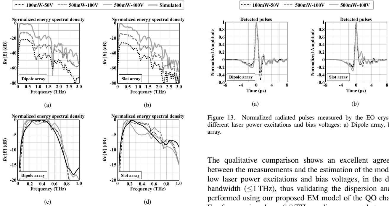
Figure 12. Normalized measured energy spectra: a)–b) Measured spectra for different bias voltages and laser power excitations on the bandwidth up to 3.0 THz, for dipole and slot array, respectively. The spectra are normalized to the maximum peak value of the spectrum with the highest energy density for both dipole and slot array, respectively. c)–d) Comparison between the normalized energy spectral densities for different bias voltages and laser power excitations, and the normalized energy spectral densities radiated by the reflectors system E_r estimated by the model on the array operative bandwidth, for the dipole and slot array, respectively. Each spectrum is normalized to the relevant maximum peak value.
