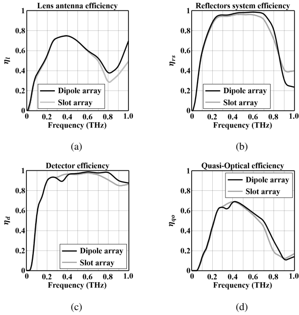
Figure 9. Simulated efficiencies of the measurement setup: a) lens antenna efficiency \eta_l ; b) reflectors system efficiency \eta_{rs} ; c) detector efficiency \eta_d ; and d) quasi-optical efficiency \eta_{qo} of the measurements setup.
