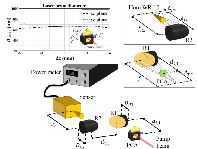
Figure 6. Measurement setup used to measure the power radiated by the photoconductive antenna prototypes, the optical system is not depicted in the figures. The geometrical features of the setup are: reflectors diameter D_{R1} = D_{R2} = 76.2 mm; reflectors f-number f_{\#1} = f_{\#2} = 2 ; distance emitter-first reflector d_{t,1} = 142.4 mm; distance second reflector-horn antenna was d_{2,r} = 142.4 mm. The top left inset shows the measured laser beam diameter at -3 dB, D_{laser} , along the horizontal (dashed line) and vertical (dotted line) planes around the position of the photoconductive source.
