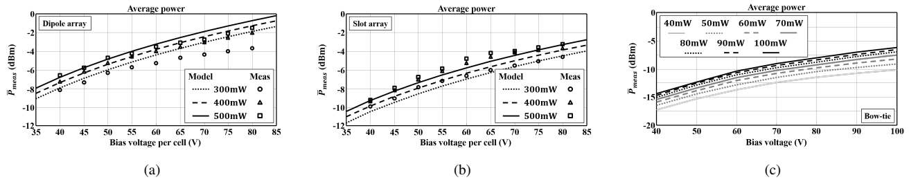
Figure 11. Measured average power and estimated average detected power \bar{P}_{meas} of the PCCA prototypes versus the bias voltage applied on the gaps: a) dipole array; and b) slot array. c) Measured average power of the bow-tie antenna versus bias voltage for different laser power excitations.
