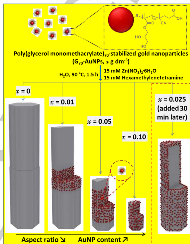
Scheme 1. Schematic representation of spatially-controlled occlusion of poly(glycerol monomethacrylate) 70 -stabilized gold nanoparticles (G 70 -AuNPs) within ZnO crystals. A twinned hexagonal rod-like ZnO crystal is obtained in the absence of any G 70 -AuNPs ( x = 0 ). In the presence of G 70 -AuNPs, shorter twinned hexagonal ZnO rods are obtained. For x = 0.01 and 0.05 , the G 70 -AuNPs are preferentially located within the central region of the rods. In contrast, uniform spatial occlusion is achieved for x = 0.10 . Finally, if the G 70 -AuNP addition is delayed for 30 min when using x = 0.025 , then only surface-confined occlusion is observed.
