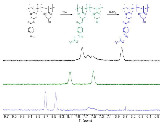
Figure 3. Stacked aromatic region of 1 H NMR spectra of the various stages of diazonium salt formation: aniline precursor (black, top), protonated aniline (green, middle) and diazonium salt (blue, bottom).
