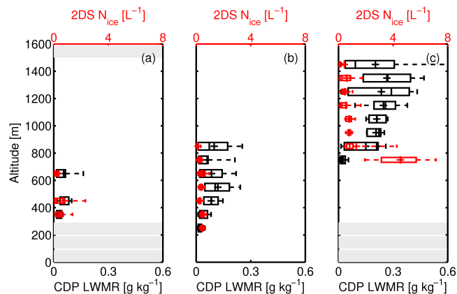
Figure 4. Observations of 2DS ice number concentration (red) and CDP liquid water mixing ratio (LWMR, black). (a) Sea ice, case 1. (b) MIZ, case 2. (c) Ocean, case 3. Only observations from mixed-phase clouds are included, with a derived CDP liquid water content threshold of \geq 0.01 \text{ g m}^{-3} distinguishing in-cloud measurements. Box edges: 25th and 75th percentiles, Median is |, and mean is +. Altitudes not sampled by the aircraft are indicated with grey boxes.
