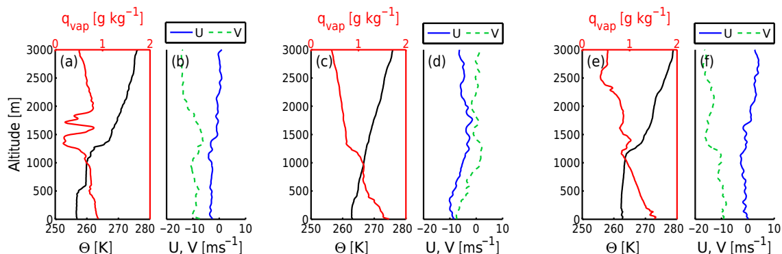
Figure 3. Potential temperature, vapour mixing ratio, and wind speed profiles measured by the three dropsondes used to initialise the LEM in this study. (a–b) Dropsonde 1 released over the sea ice during flight B762. (c–d) Dropsonde 2 released over the MIZ during flight B764. (e–f) Dropsonde 3 released over the ocean during flight B762.
