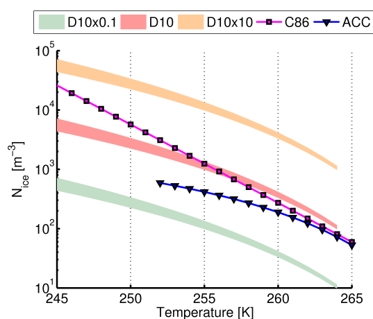
Figure 1. Evaluation of the five parameterisations used (C86, D10, ACC, \text{D10} \times 0.1 , and \text{D10} \times 10 ) in the three cases considered with respect to temperature. The C86 parameterisation and ACC are valid for all cases, whereas the different aerosol particle loadings, and thus, variability, are accounted for with the D10 parameterisation.
