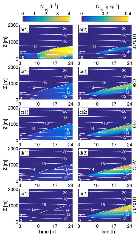
Figure 9. MIZ (case 2) simulations, presented similarly to Fig. 6.
