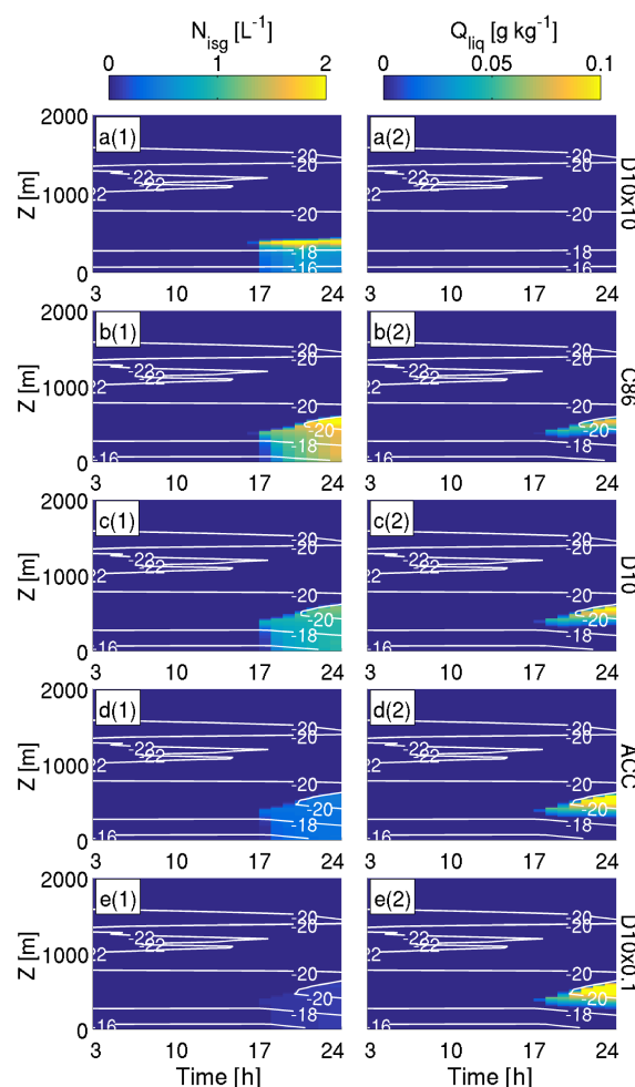
Figure 6. Simulated total ice number concentrations ( N_{\text{ice}} , a1–e1 ) and liquid water mixing ratios ( Q_{\text{liq}} , a2–e2 ) using the (a) \text{D10} \times 10 , (b) C86, (c) D10, (d) ACC, and (e) \text{D10} \times 0.1 parameterisations for case 1 (sea ice). All are restricted to water saturation. Run length 24 h. Temperature ( ^{\circ}\text{C} ) contours are overlaid in white. Runs are arranged such that the simulation which produced the most ice ( \text{D10} \times 10 , a) is on the top row, and that which produced the least ice ( \text{D10} \times 0.1 , e) is on the bottom row. Note the changing colour bar at the top of each column, which corresponds to data in that column only.
