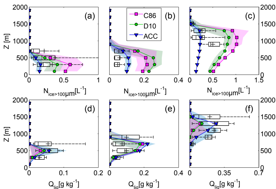
Figure 7. Observed N_{\text{ice} > 100\mu\text{m}} and Q_{\text{liq}} for the sea ice (column 1), MIZ (column 2), and ocean (column 3) cases. Observations are shown as black boxes, similar to Fig. 4. Mean modelled concentrations of ice and snow particles greater than 100\mu\text{m} , using the C86 (magenta), D10 (green), and ACC (blue) parameterisations, are overlaid. Model time steps of 21, 17, and 7 h are used for the sea ice, MIZ, and ocean cases respectively, as these time steps offer the best comparison with the observations. Shading (in pink, green, or blue for C86, D10, and ACC respectively) indicates variability in the model parameters from \pm 3\text{h} in cases 1 and 2, and \pm 4\text{h} in case 3, where a larger interval is implemented in the latter case as the chosen parameters showed little variability over the shorter time step. In panel (f), the variability illustrated is always less than the mean modelled profile shown using each parameterisation as the Q_{\text{liq}} is at its greatest at the chosen time step. Observed N_{\text{ice} > 100\mu\text{m}} data from noted shattering event (Young et al., 2016a) are excluded in panel c, so that only primary contributions of ice are considered.
