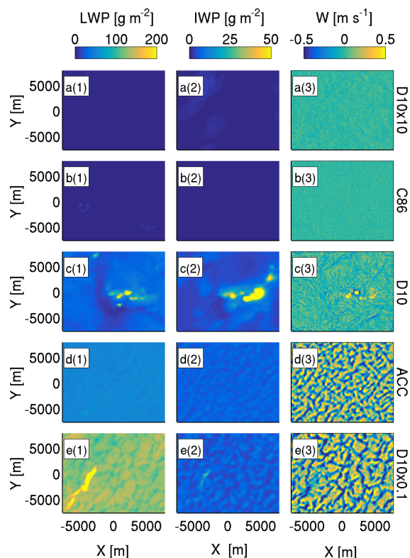
Figure 11. LWP (a1–e1), IWP (a2–e2), and vertical velocity ( W , a3–e3) at approximately 1500 m for each simulation in the ocean case. Planar X - Y slices are shown at 21 h. Note changing colour bar at the top of each column, which corresponds to data in that column only.
