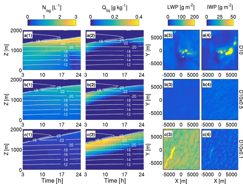
Figure 13. N_{\text{isg}} (a1–c1), Q_{\text{liq}} (a2–c2), LWP (a3–c3), and IWP (a4–c4) modelled in the (a) D10, (b) D10 \times 0.5 , and (c) D10 \times 0.1 simulations over the ocean (case 3). Data are presented similarly to Figs. 10 and 11. Temperature ( ^{\circ}\text{C} ) contours overlaid in white in panels 1 and 2. Note changing colour bar at the top of each column, which corresponds to data in that column only.
