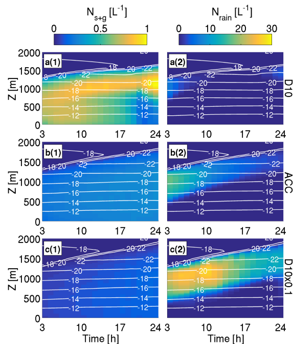
Figure 12. Summed snow and graupel number concentrations ( N_{s+g} , a1–c1) and rain number concentration ( N_{rain} , a2–c2) using (a) D10, (b) ACC, and (c) D10 \times 0.1 during case 3. Run length 24 h. Temperature ( ^{\circ}C ) contours are overlaid in white. Note changing colour bar at the top of each column, which corresponds to data in that column only.
