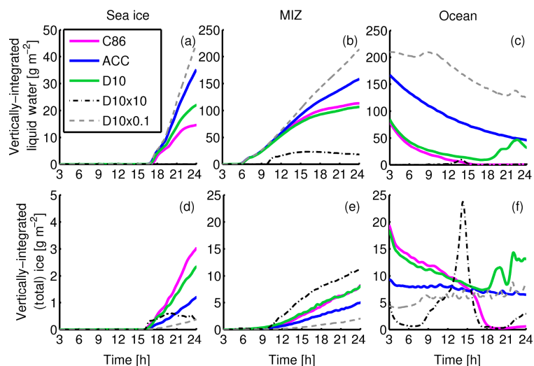
Figure 8. Vertically integrated liquid (a–c) and ice water paths (d–f) for the sea ice, MIZ, and ocean cases when implementing each of the C86, ACC, D10, D10 \times 10 , and D10 \times 0.1 parameterisations under water-saturated conditions.
