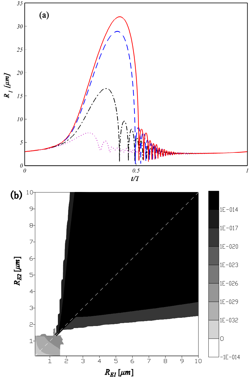
Figure 6: (a) The radius R_1(t) for bubbles with (R_{E1}, R_{E2}) = (3, 4)\mu\text{m} , calculated with D = 0.1\text{mm} and p_a = 1.32p_{\text{atm}} . From the top to bottom, \eta = 0, 1, 5, 10\text{KPa} . (b) The force factor f_{12} for the KV fluid (lower half) with \eta = 5\text{KPa} and the Newtonian fluid (upper half). p_a = 1.42p_{\text{atm}} . f = 20\text{KHz} . D = 100\mu\text{m} .
