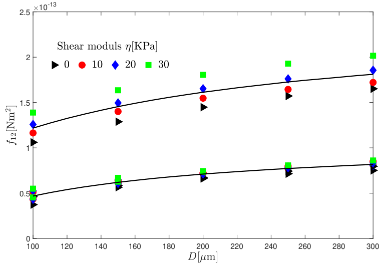
Figure 8: f_{12} versus D . Top group: (R_{E1}, R_{E2}) = (6, 8) \mu\text{m} . Bottom group: (4, 6) and (4, 8) \mu\text{m} . Solid lines: the average in each group. Calculated with matching pressure for p_a^N = 1.32 p_{\text{atm}} , f = 20 \text{KHz} .
