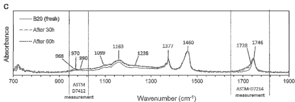
Figure 2. Comparison of FT-IR spectra from fresh and aged oils samples; a) JO; b) EMO; and c) B20.
