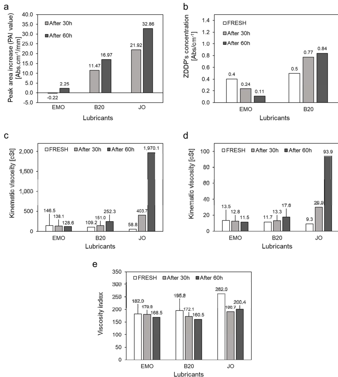
Figure 3. Oxidation and changes in viscosity for the fresh and aged oil samples: a) PAI values; b) ZDDP concentration; c) kinematic viscosities obtained at 26 °C; d) kinematic viscosities obtained at 100 °C; e) viscosity index.
