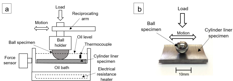
Figure 1. a) Schematic representation of the reciprocating friction test set-up; b) steel ball and cylinder liner specimens.
