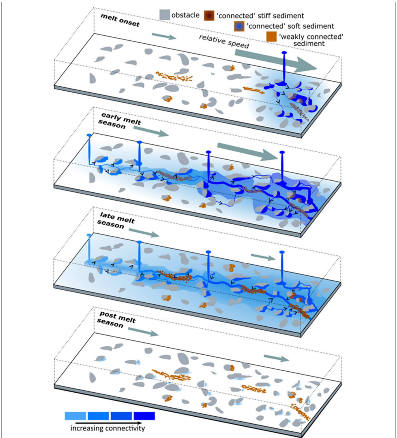
FIGURE 8 | Conceptual model of land-terminating Greenland Ice Sheet seasonal hydrology and dynamics. Melt onset activates part of the weakly-connected drainage system (white background) and subsequent fluctuations in runoff supply lead to cavity expansion, increased sediment deformation and consequent rapid speed-up (grey arrow). In the early-melt season, meltwater accesses the bed at progressively higher elevations and the efficiency and extent of the connected drainage system increases (blue shading), likely forming channels at lower elevations. Surface runoff supply frequently exceeds the capacity of the core of the connected drainage system at progressively higher elevations during the early-melt season, causing speed-up. During the late-melt season, runoff supply declines, and water drains across variable pressure axes and from the weakly-connected system toward efficient drainage forms at lower elevations, but not higher elevations, where drainage system efficiency remains low throughout the melt season. Basal water pressure and cavity size gradually increase during the post-melt season.
