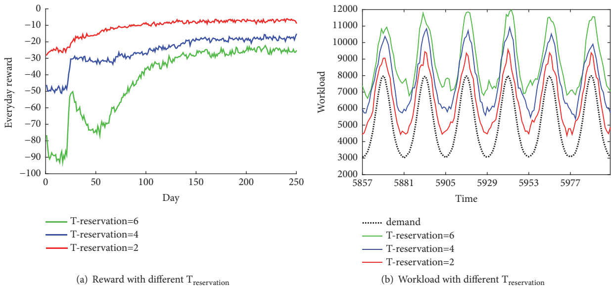
FIGURE 7: Comparison results regarding different T_{reservation} .
