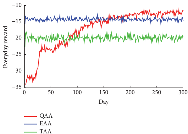
FIGURE 8: Performance comparison in reserved VMs market.
