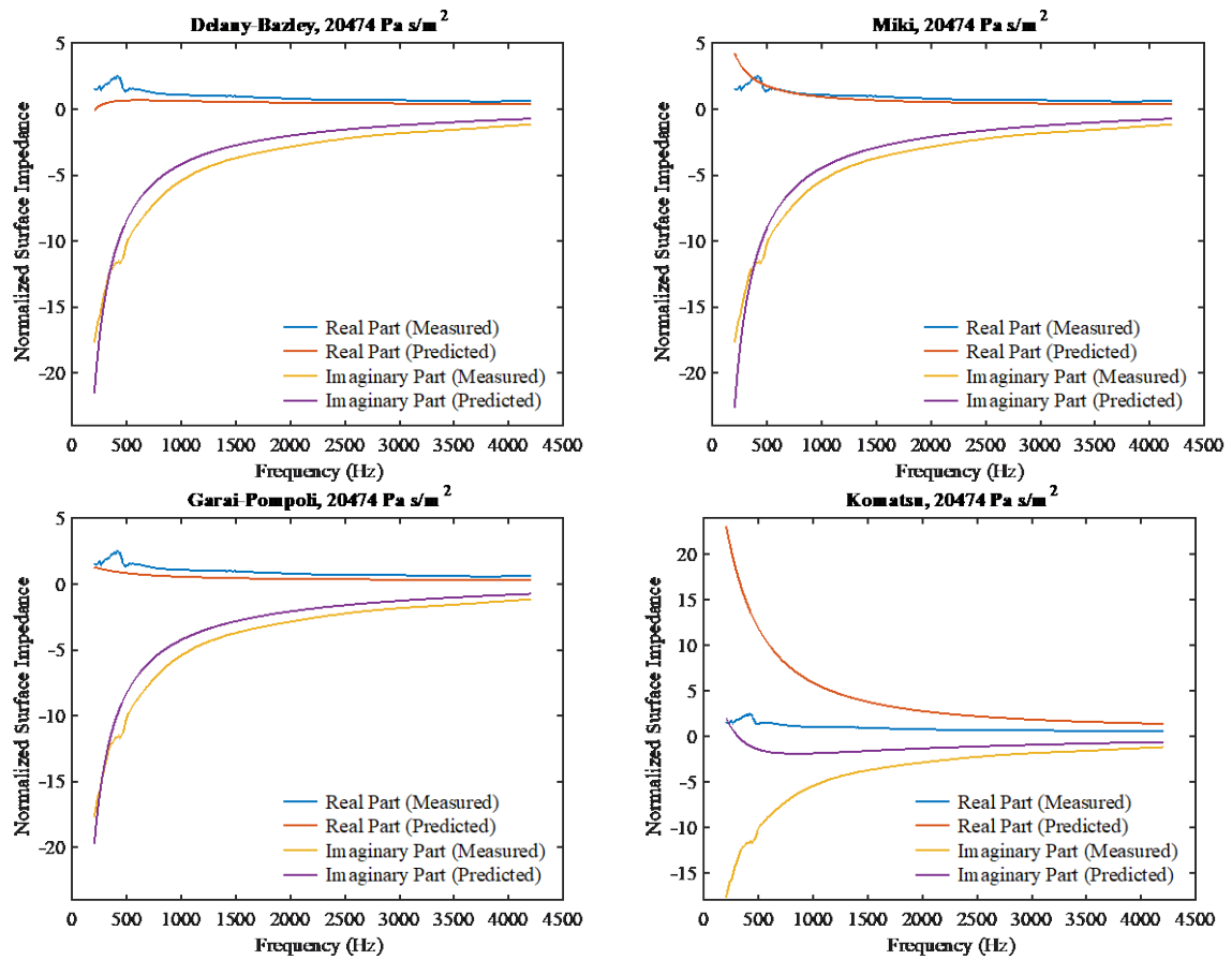
Figure C5. Measured and predicted impedance for the sample with airflow resistivity of 20474 \text{ Pa}\cdot\text{s}/\text{m}^2 .
