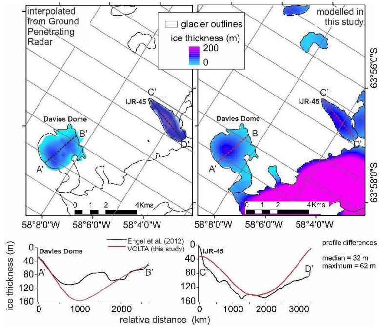
898 Figure 3. Comparison of ice thickness modelled in this study with that from Engel et al. (2012) who 899 interpolated between ground penetrating radar data on Davies Dome ice cap and IJR-45 valley glacier, 900 both on the Ulu Peninsula on James Ross Island. The ice thickness transects are chosen to closely 901 follow GPR lines so as to exclude interpolation error from these transect comparisons. 902
