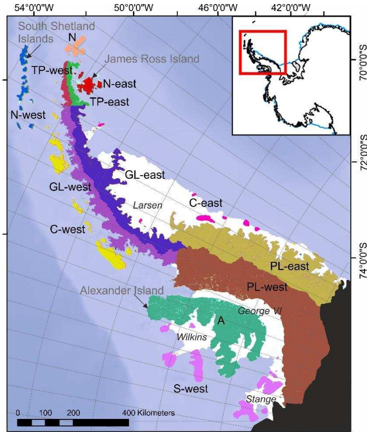
876 Figure 1. Major glacier regions across the Antarctic Peninsula as used in this study to spatially 877 discriminate ice thickness, bed topography, ice volume and potential sea level contributions. 878 Surrounding islands are grouped spatially and the labelled codes for these groups are expanded in 879 Table 1 .
