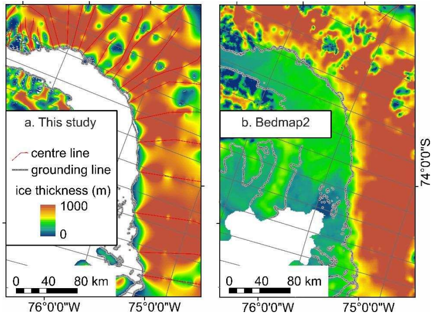
884 Figure 2. Example of multiple centrelines per single glacier outline artificially introduced to 885 accommodate application of the VOLTA model to wide, low-angle and coalescing glaciers that are 886 typical of the southern part of the Antarctic Peninsula, in this case on the mainland opposite the south 887 coast of Alexander Island. The resultant VOLTA-computed ice thickness (A) matches the magnitude 888 and spatial pattern of ice thickness from Bedmap2 (B) well. Grounding lines are from Rignot et al. 889 (2011). Bedmap2 data is from Fretwell et al. (2013).
