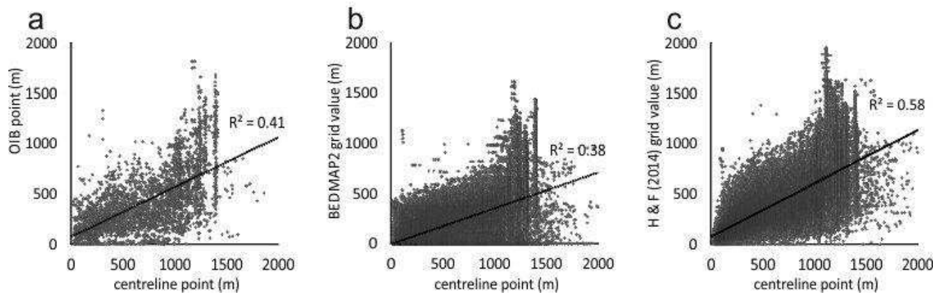
914 Figure 5. Cross-over analysis of ice thickness for our modelled glacier centreline points ( n = 81,463 ) 915 and closest (if within 500 m) Operation Ice-Bridge (2016) points (a). For comparison, the 916 corresponding ice thickness grid cell values of Bedmap2 (Fretwell et al., 2013) ice thickness and Huss 917 and Farinotti's (2014) ('H&F') ice thickness at each of these centreline points are also shown in panels 918 b and c, respectively.
