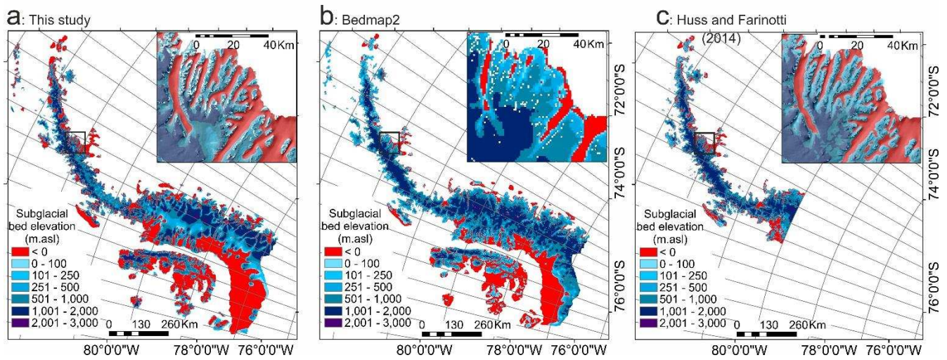
986 Figure 10. Subglacial topography, emphasizing those areas of the Antarctic Peninsula that are below 987 sea level and so potentially contribute by a relatively small amount to sea-level rise, as modelled by this 988 study (a) within the Bedmap2 (Fretwell et al., 2013) dataset (b) and as modelled by Huss and Farinotti 989 (2014) (c). Note that the insets in panels a and b are underlain by hillshaded bed topography for clarity 990 of the 100 m resolution grid.
