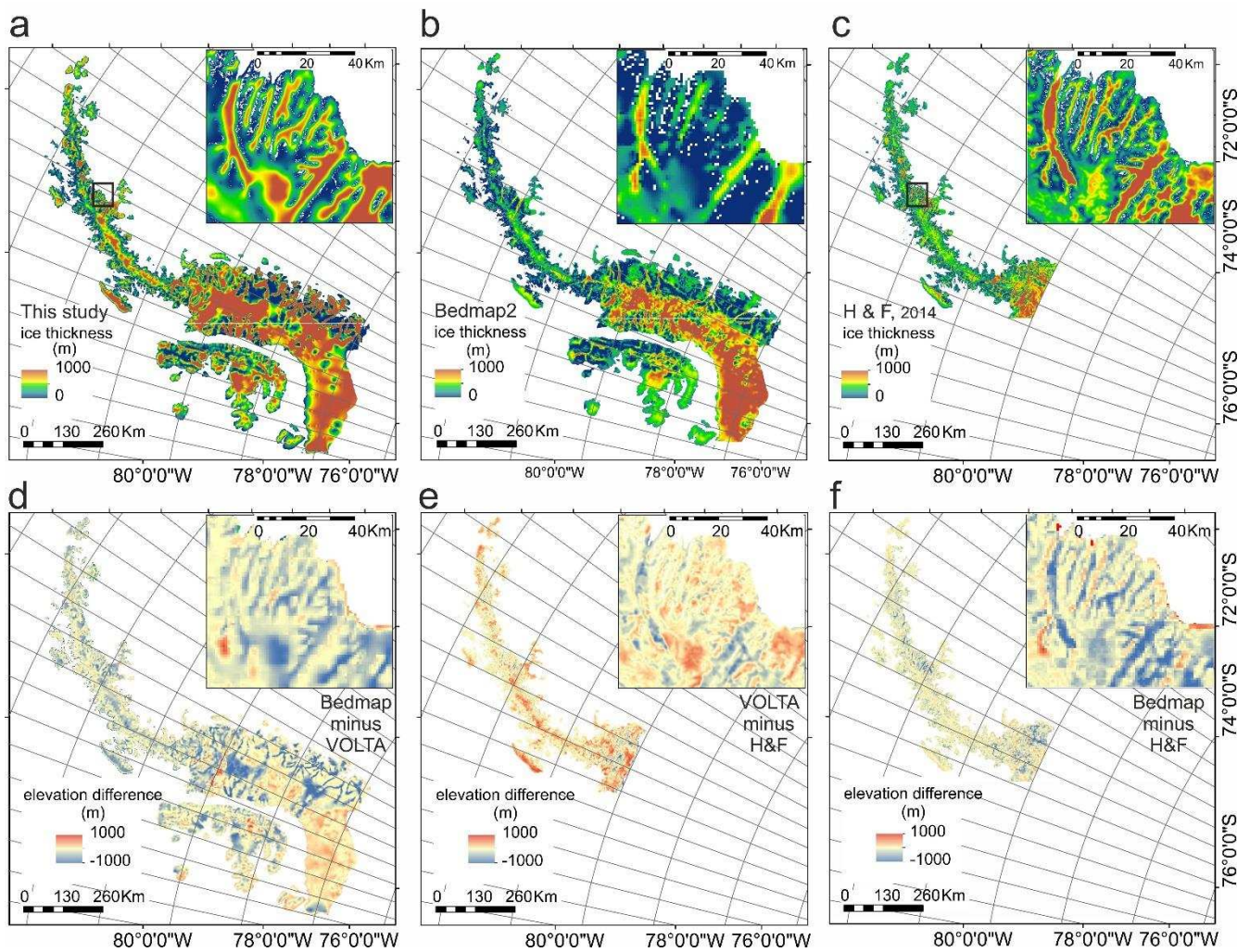
959 Figure 8. Gridded ice thickness modelled in this study (a) the Bedmap2 (Fretwell et al., 2013) dataset 960 (b), and modelled by Huss and Farinotti (2014) ('H&F') (c). Differences in ice thickness between 961 Bedmap2 and this study, between Huss and Farinotti and this study, and between Huss and Farinotti 962 and Bedmap2 are shown in panels d, e and f, respectively. Colour scales are identical in all panels and 963 in all insets. Inset is chosen to be same area as emphasised by Huss and Farinotti for its subglacial 964 trough topography.
