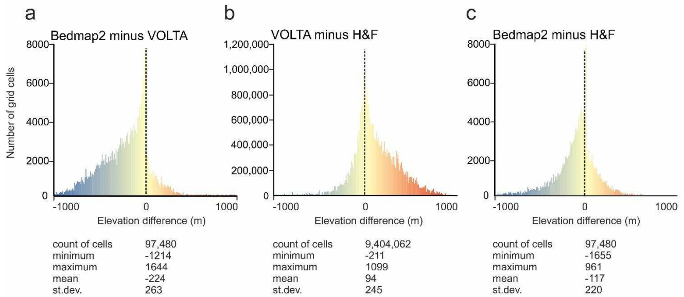
968 Figure 9. Histogram comparison of grid cell values between the modelled ice thickness of this study 969 and Bedmap2 (a), between this study and the ice thickness modelled by Huss and Farinotti (2014) 970 ('H&F') (b) and Huss and Farinotti and Bedmap2 (c). Bars are coloured to match the elevation 971 differences as mapped in Figure 4 .
