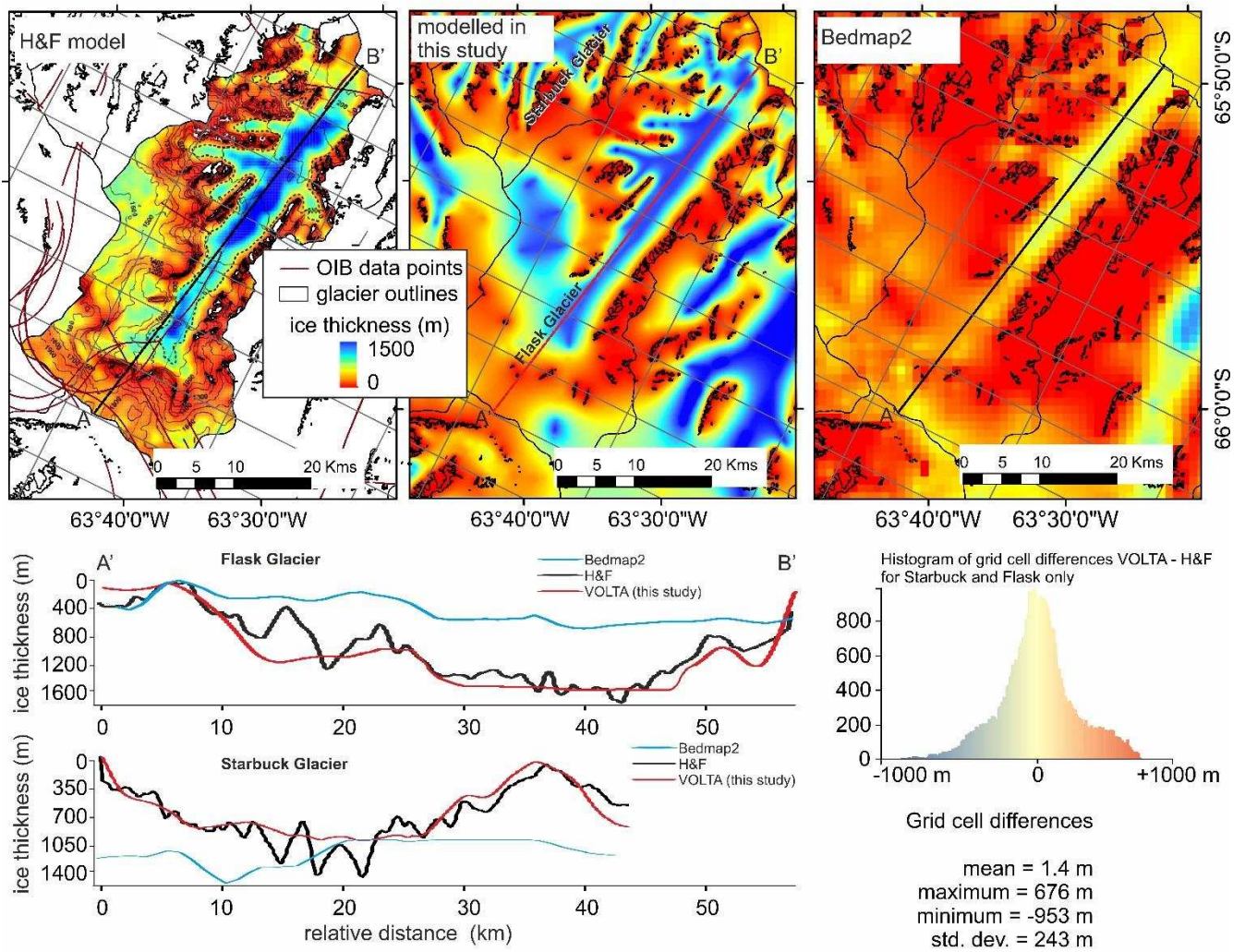
904 Figure 4. Comparison of ice thickness modelled in this study with that from Farinotti et al. (2013, 905 2014) who optimised their ice thickness model using ground penetrating radar data and ice velocity 906 data on Flask Glacier and on Starbuck Glacier, both of which are tidewater glaciers. The glacier outline 907 at the end of the transect and at point B' is determined by the grounding line, as mapped by Rignot et 908 al. (2011).
