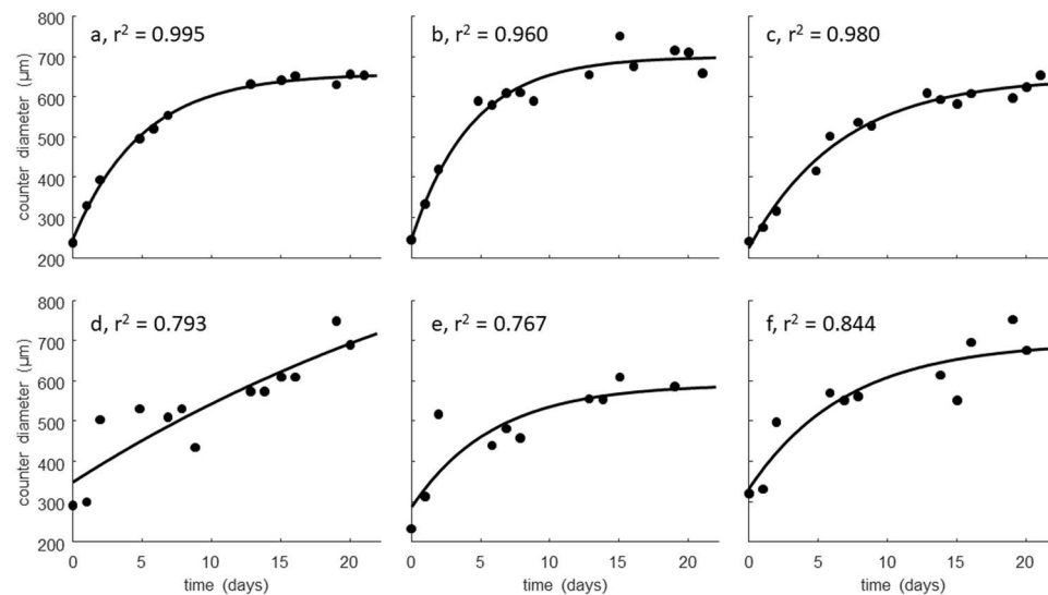
Figure 3. Examples of von Bertalanffy growth curves [L(t) = L_{\infty} - (L_{\infty} - L_0) \exp(-rt)] fitted to body size measured over time for individual daphnids ( C. dubia ). Top figures show excellent (a) to good (b,c) fits, whereas the bottom row shows some very poor fits (d–f).
