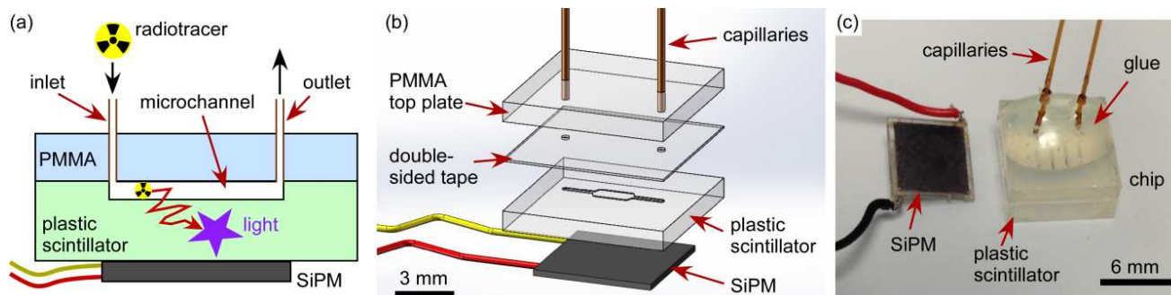
Figure 1. (a) Design principle of the microfluidic radio-HPLC detector fabricated from plastic scintillator. When a positron-emitting radioisotope (e.g. [ ^{18}\text{F} ]fluoride) is injected into the device the positrons interact with the scintillator, generating light that is detected with a silicon photomultiplier (SiPM). (b) Exploded schematic of the microfluidic device consisting of a milled scintillator layer bonded to a PMMA top plate, with the SiPM placed below the chip. (c) Photograph of the assembled microfluidic device alongside a SiPM.
