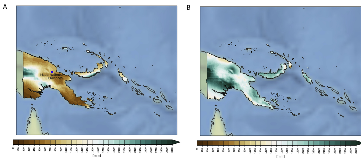
Fig. 6. Seasonal rainfall totals in Papua New Guinea for (a) the MJJASO (dry) season (left panel), (b) the NDJFMA (wet) season (right panel) averaged over the 1981–2010 period. Data from the MSWEP dataset (Beck et al., 2017) (Source: Met Office).
