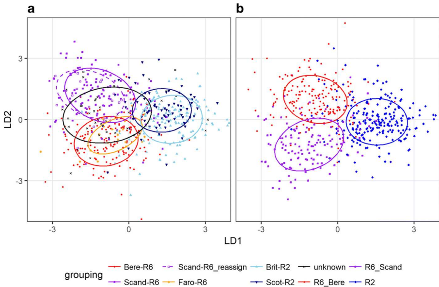
Fig. 2 Linear discriminant analysis (LD1 and LD2) of GMM data for barley grains. a 525 grains from the 50 accessions with non-anomalous SNP data, assigned according to accession information with the 20 grains from the four unknown accessions added as new data. b 525 grains from the 50 accessions with non-anomalous SNP data, assigned according to genetic cluster. Confidence ellipses set at level 0.68. Symbols (and colours and ellipse lines) denote barley group: a circle (red)—six-row bere; filled square (purple)—six-row Scandinavian; open square (purple, dashed ellipse line)—presumed six-row Scandinavian; upward triangle (light blue)—two-row non-Scottish British; downward triangle (dark blue)—two-row Scottish; star (orange)—six-row Faroese; multiplication sign (black)—six-row unknown origin; b Circle (red)—six-row bere or Faroese; squares (purple) six-row Scandinavian including presumed Scandinavian; diamonds (blue)—two-row British
