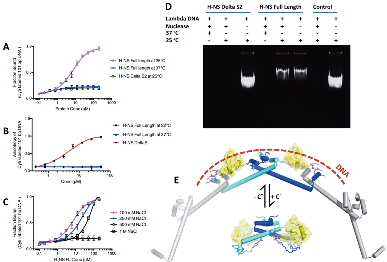
Figure 6. H-NS:DNA interactions are incompatible with the H-NS N/C association. Interactions between H-NS FL and H-NS \Delta S2 with 101bp DNA were determined using (A) MST and (B) fluorescence anisotropy. (C) Influence of NaCl on the interaction between H-NS FL with 101bp DNA, determined using MST. Data in (A–C) are means \pm S.D., n = 3 . (D) Nuclease assay of lambda DNA in the presence of H-NS FL and H-NS \Delta S2 under different conditions. (E) Proposed temperature switch mechanisms. Top : Under conditions where site2 dimers are stable, H-NS will multimerize. In this conformation, the linker residues (magenta), DNAbd (yellow) and positive charges on site1 (stick representation) of linked H-NS molecules can cooperate to achieve a strong association with DNA (indicated as dashed line). Bottom : Under conditions where site2 unfolds, the C-terminal linker and DNAbd associate with the N-terminal site1, leading to an autoinhibited dimeric conformation incapable of DNA binding and of formation of higher-order multimers. Although based on experimental data, the positions of the acidic linker and DNAbd are speculative.
