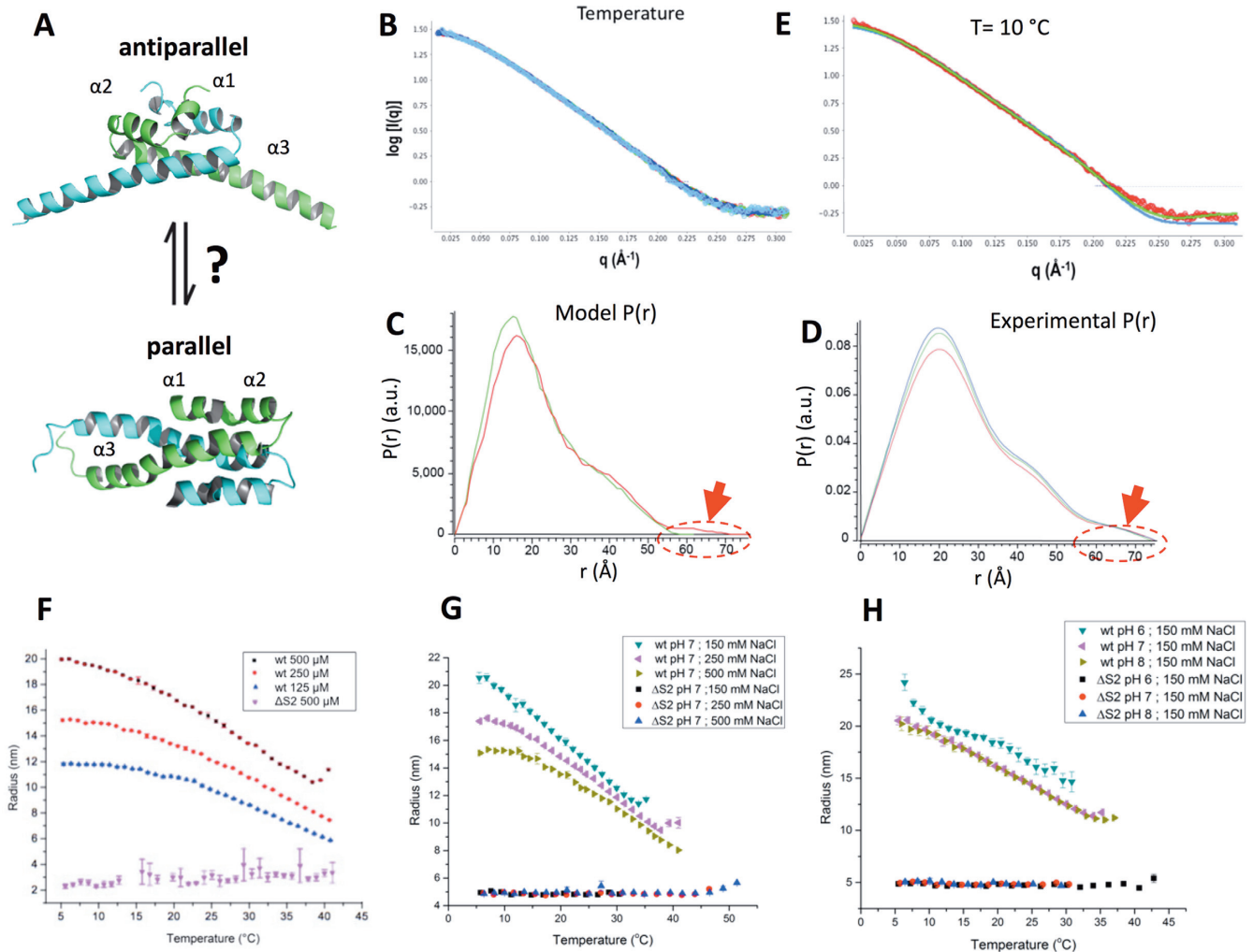
Figure 2. Environmental influence on the structure of S. typhimurium H-NS. (A) Structural models for site1 (residues 1–57 are shown). Top : antiparallel model, as observed in E. coli H-NS 1–46 (1NI8, NMR), S. typhimurium H-NS 1–83,C21S (3NR7, X-ray), S. typhimurium H-NS 1–46 (4ICG, X-ray) and V. cholerae VicH 1–48 (1OV9, X-ray). bottom : parallel model, as determined for S. typhimurium H-NS 1–57,C21S (1LR1, NMR). The two chains of each dimer are coloured green and cyan. (B) Superimposed are SAXS data collected on S. typhimurium H-NS 2–57,C21S at 10°C (light blue), 20°C (dark blue), 30°C (green) and 42°C (red). Data were collected in 150 mM NaCl, 1 mM EDTA, 20 mM Tris pH 7.5. (C) Pair distance distributions P(r) calculated for the parallel (green) and antiparallel (red) models for H-NS 1–57,C21S . The encircled area and red arrow highlight a main difference between the both site1 models. (D) P(r) for H-NS 2–57,C21S , derived from SAXS data shown in (D); 20°C (blue), 30°C (green) and 42°C (red). (E) Fit of calculated SAXS pattern (green) to experimental data (red dots) collected at 10°C. Green: antiparallel model; \chi^2 = 2.22 . Blue: parallel model; \chi^2 = 7.56 . Fits were calculated by FoXS (57). (F–H) DLS measurements of R_H as a function of temperature. (F) Temperature and concentration dependence of multimerization of H-NS without fused mCherry. Wt: full-length H-NS; \Delta S2 : H-NS \Delta s2 . (G) Influence of salt on multimerization of m^{Ch} H-NS (wt) and m^{Ch} H-NS \Delta s2 ( \Delta S2 ). (H) as (G) but with variations in pH. For other salt and pH scans, please see Supplementary Figure S3. Data in (F–H) are means \pm S.D., n = 3 .
