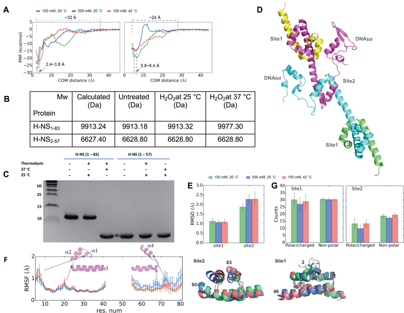
Figure 3. Site2, but not site1, of S. typhimurium H-NS is sensitive to changes in temperature and salinity. (A) PMF plots of site1 (left) and site2 (right) dimers along the pulling direction using COM distance between two monomers as the collective variable. The dissociation state of the monomers is set as the reference (0.0 kcal/mol) for each calculation. We averaged the data with SDs as error bars from six PMFs; the small standard deviations (SDs) indicate the convergence of the PMF. (B) Molecular weight determination of H-NS 1-83,C21S or H-NS 2-57,C21S at different temperatures in the presence or absence of hydrogen peroxide (H 2 O 2 ). Calculated Mw for unmodified proteins includes leftover of cleavage from tags (H-NS 1-83,C21S : residues GPLGS; H-NS 2-57 : GS). (C) Proteolytic cleavage of H-NS 1-83 or H-NS 2-57 with thermolysin at different temperatures. (D) A final snapshot of the full-length H-NS dimer (centre), and superimposed site1 (top) and site 2 (bottom) structures under regular, salt, and heat conditions taken from 200 ns MD simulations. (E) Histogram of C \alpha RMSD of site1 and site2 dimers, with the S. typhimurium H-NS crystal structure (PDBID: 3NR7) as the reference. We superposed residues 5–41 and residues 55–81 for the RMSD calculations of site1 and site2, respectively. (F) Plot of average residue fluctuation (RMSF) for site1 and site2 with respect to the crystal structure (PDBID: 3NR7), presented along the H-NS sequence. Prominent features the high-temperature and high-salinity conditions are highlighted in red and blue, respectively. (G) Histograms of the polar(H-bond)/charged(ionic) contacts and of non-polar(hydrophobic) contacts across protein chains of site1 and site2 dimers. The data in (E) and (G) were averaged with SDs as error bars from all replica simulations.
