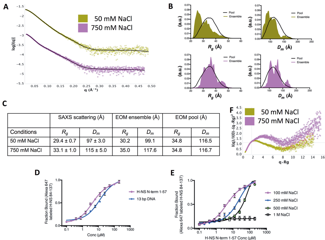
Figure 4. H-NS \Delta s2 adopts a relatively compact conformation in vitro. (A) Experimental H-NS \Delta s2 SAXS patterns recorded at 50 mM NaCl (green) and 750 mM NaCl (pink). Calculated SAXS pattern from ensemble models are shown in black. The corresponding Guinier plots are shown in Supplementary Figure S8. (B) Histogram of R_g and D_m for pool (black line) and selected ensemble models (olive for 50 mM NaCl data, and pink for 750 mM NaCl data). a.u.: arbitrary units. The corresponding ensemble models are shown in Supplementary Figure S8. (C) R_g and D_m values calculated from (A) and (B) are tabulated. (D) Interactions of fluorescently labeled H-NS _{84-137} with H-NS _{1-57} and 13bp DNA determined using MST. (E) Influence of NaCl on the H-NS _{84-137} :H-NS _{1-57} interaction determined using MST. Data in (D, E) are means \pm S.D., n = 3 .
