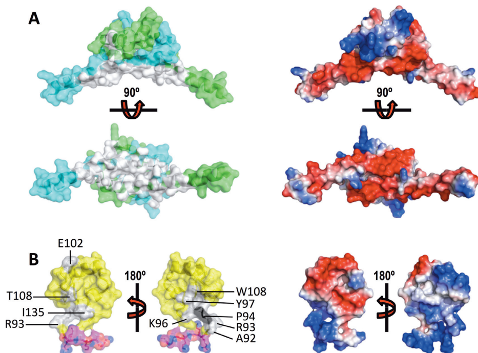
Figure 5. The H-NS C-terminal region binds to the N-terminal domain. (A) Left: Chemical shifts (grey) mapped on H-NS 2-57 chains A (green) and B (cyan). right: electrostatic surface of H-NS 2-57 . Top and bottom panels show 90° views. (B) Left: Chemical shifts (grey) mapped on H-NS 84-137 . Proline 94 is shown in black. Yellow: DNAbd; magenta: linker residues 84–90. Right: electrostatic surface of H-NS 84-137 . For each representation, 180° views are shown, as indicated.
