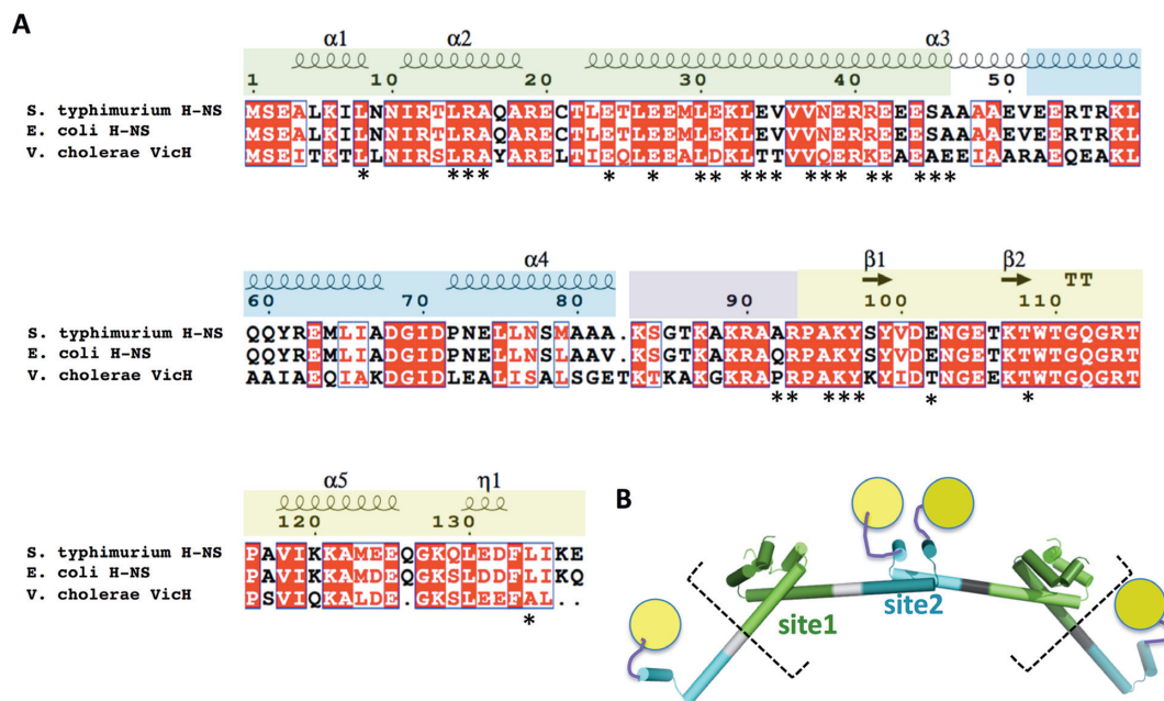
Figure 1. Domain organization of H-NS. (A) Sequence alignment showing structural elements ( \alpha -helices, \beta -strands; \eta represents a 3_{10} helix). Protein domains (determined from experimental structures) are green: N-terminal dimerization domain (site1); blue: central dimerization domain (site2), purple: positively charged linker; yellow: C-terminal DNA binding domain (DNABd). Positions of S. typhimurium residues showing chemical shift changes in presence of H-NS 84-137 or H-NS 2-57 are indicated by an asterisk. (B) Schematic structural model for multimerization through site1 (light and dark green) and site2 (light and dark cyan) extracted from the H-NS superhelix conformation (see (35) and PDB 3NR7). The charged linker (purple) and DNABd (yellow) are not included in the crystallographic model. Dashed square brackets outline the construct used in MD simulations.
