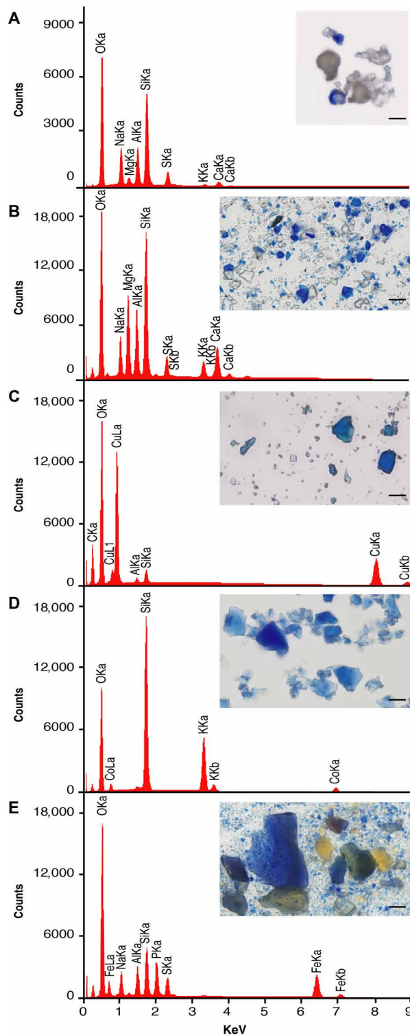
Fig. 3. Elemental composition of archaeological blue particle and blue reference pigments measured by EDS. (A) Blue particle isolated from medieval dental calculus. (B) Afghan lazurite reference pigment (RC, 410-15). (C) Azurite reference pigment (RC, 410-10). (D) Smalt reference pigment (RC, 417-14). (E) Vivianite reference pigment (RC, 410-20). The archaeological blue particles lack copper (Cu), cobalt (Co), and iron (Fe) but closely match the spectrum produced by the tectosilicate lazurite. Scale bars, 20 \mu\text{m} . Additional reference spectra are provided in fig. S7. Raw data are provided in data file S2. Credit: M. Tromp.
