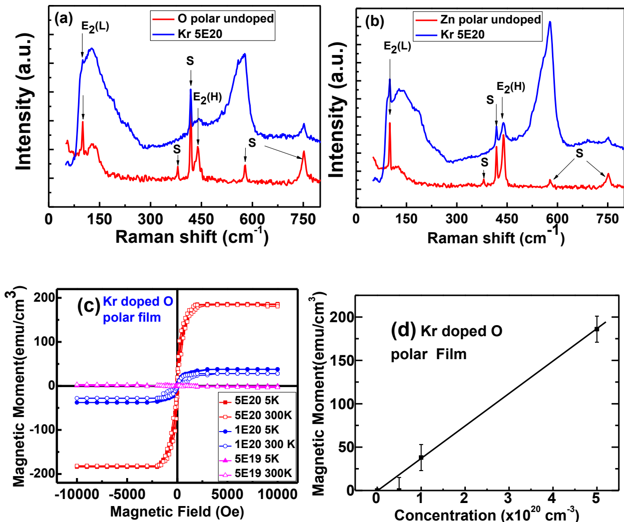
Fig. 5 (color online) Raman spectra for the undoped (red) and 5 \times 10^{20}\text{ cm}^{-3} Kr doped (blue) ZnO films. (a) O polar (b) Zn polar films and (c) M-H loops for the O-polar film
